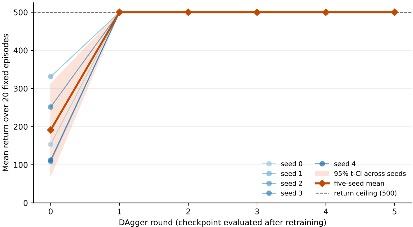
CartPole-v1: independent training seeds with common evaluation episodes
