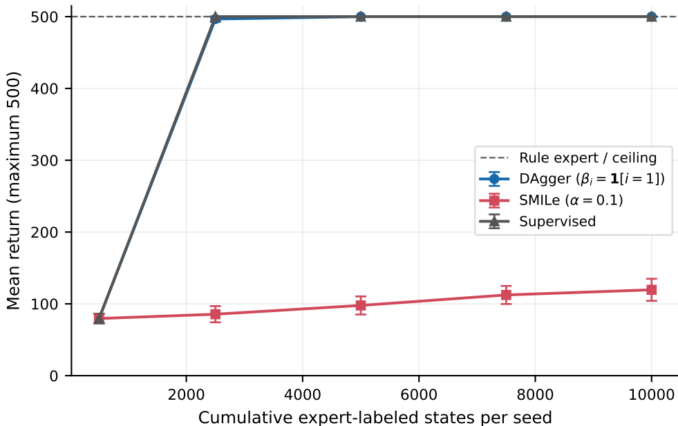
CartPole return at paper-matched checkpoints
