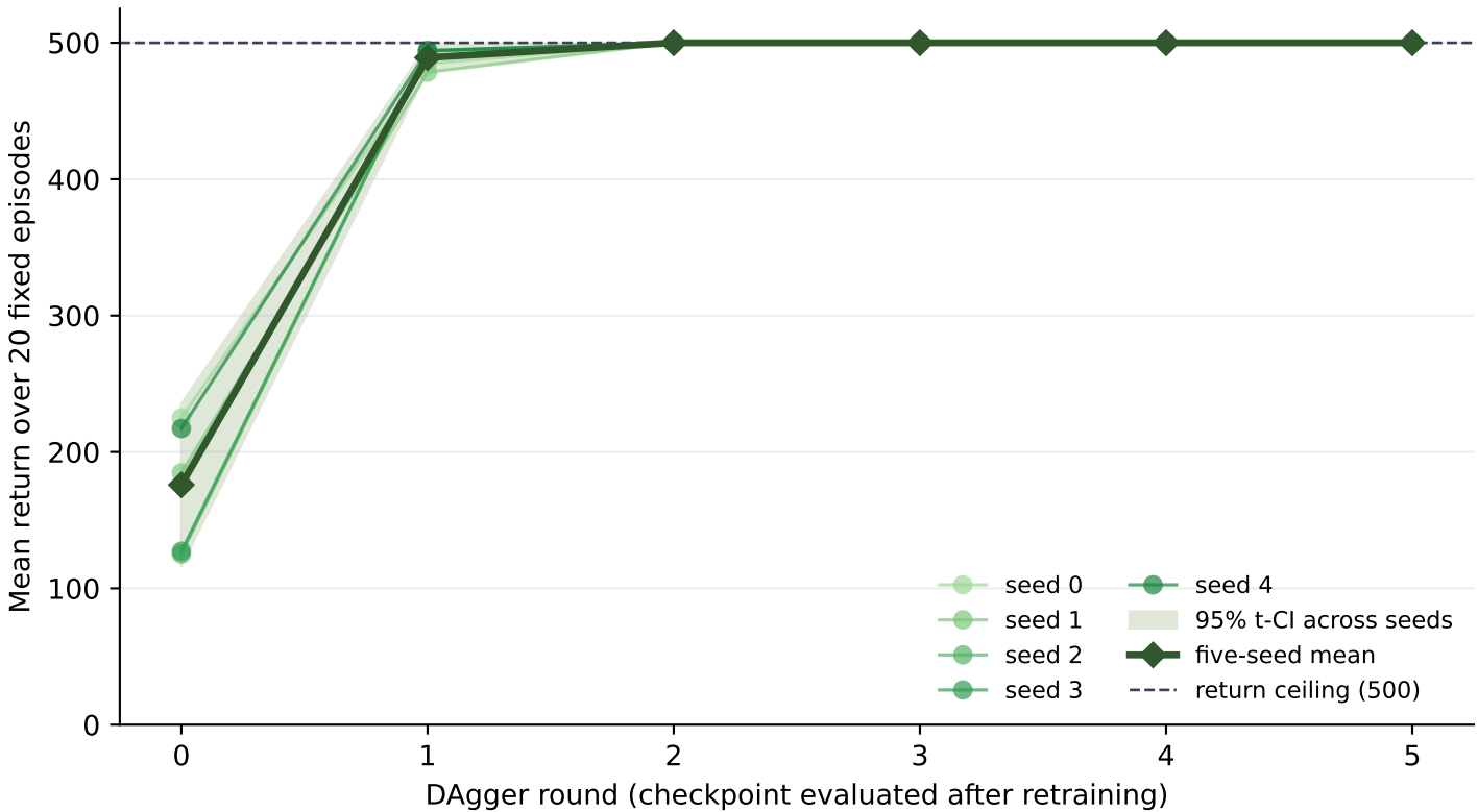
CartPole-v1 rule expert: five independent learner seeds
