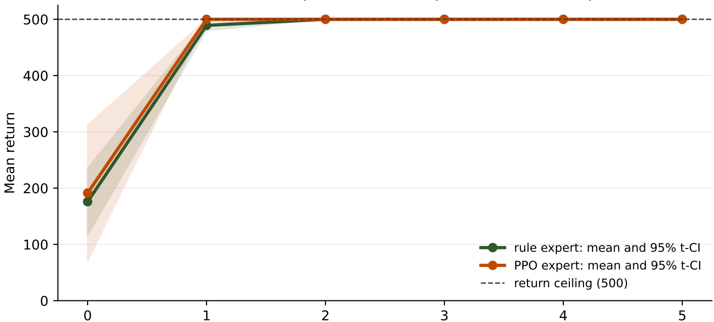
Zoom: convergence at rounds 1--2
