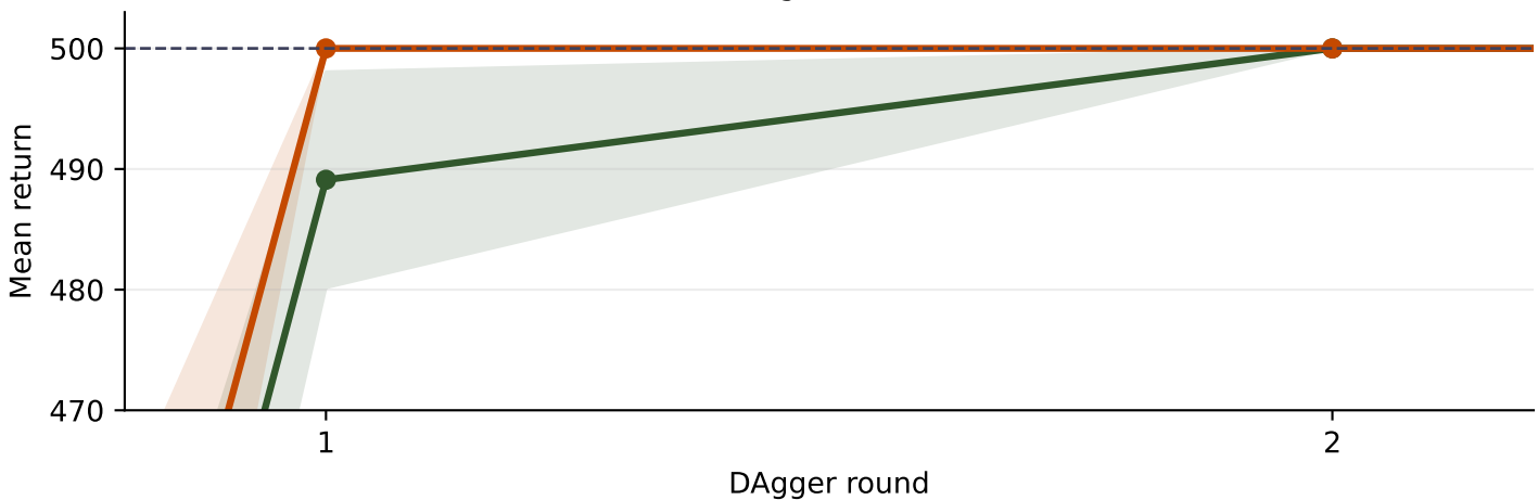
Zoom: convergence at rounds 1--2
