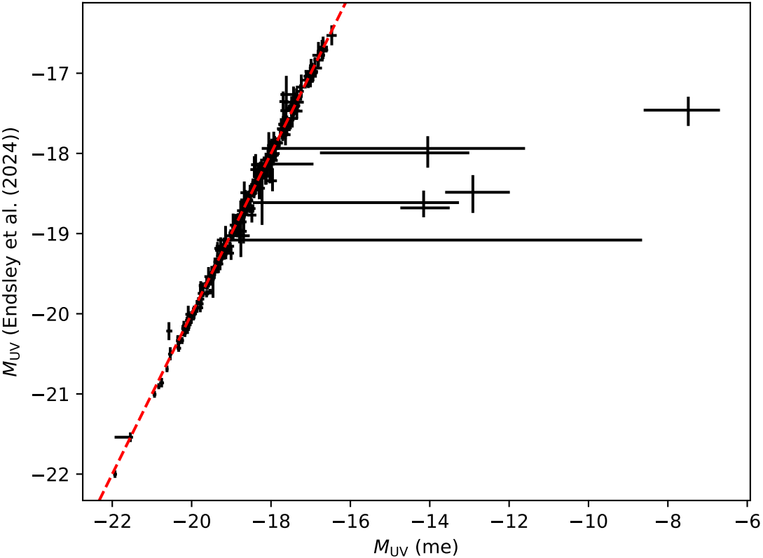
Comparing M_{UV} measurements of the F775W dropouts from Endsley et al. (2024)
