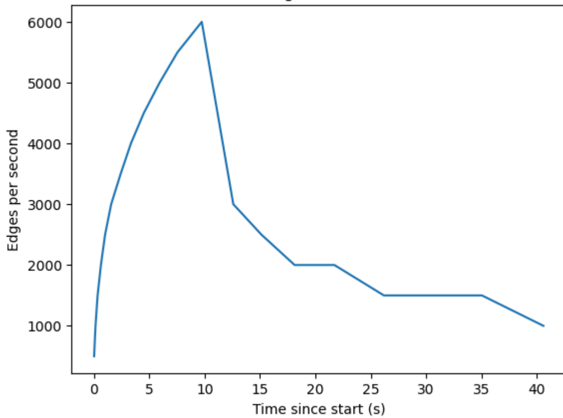
Sliding-window EPS
