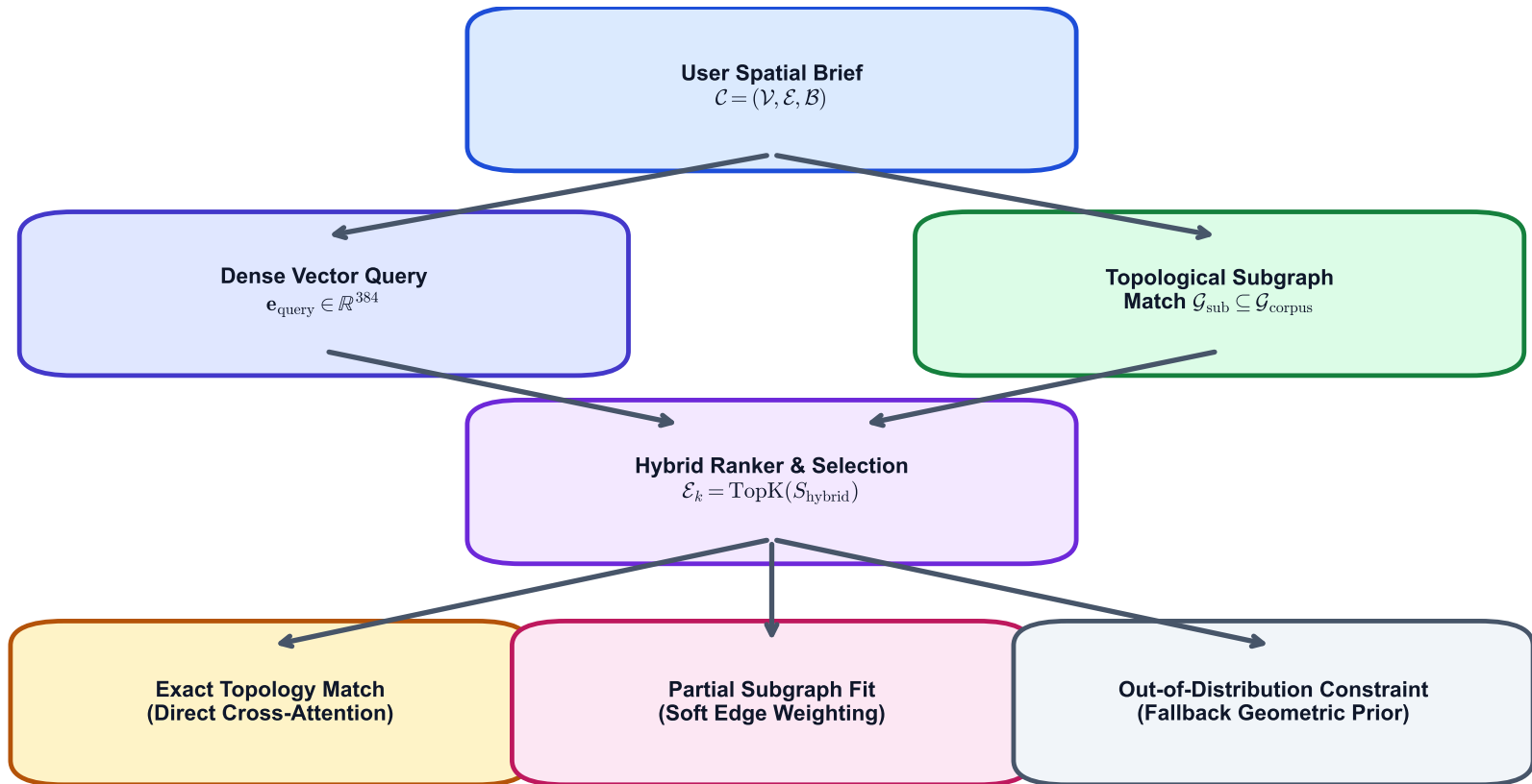
Figure 3: Algorithmic Adjacency Contingency & Dual Index Resolution Tree
