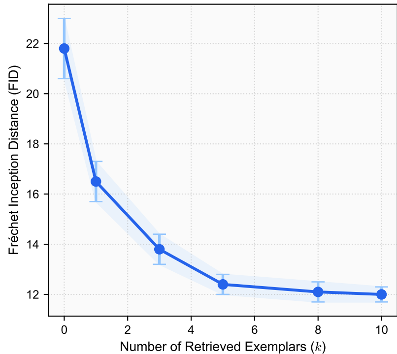
(c) FID Sensitivity vs Exemplar Count k
