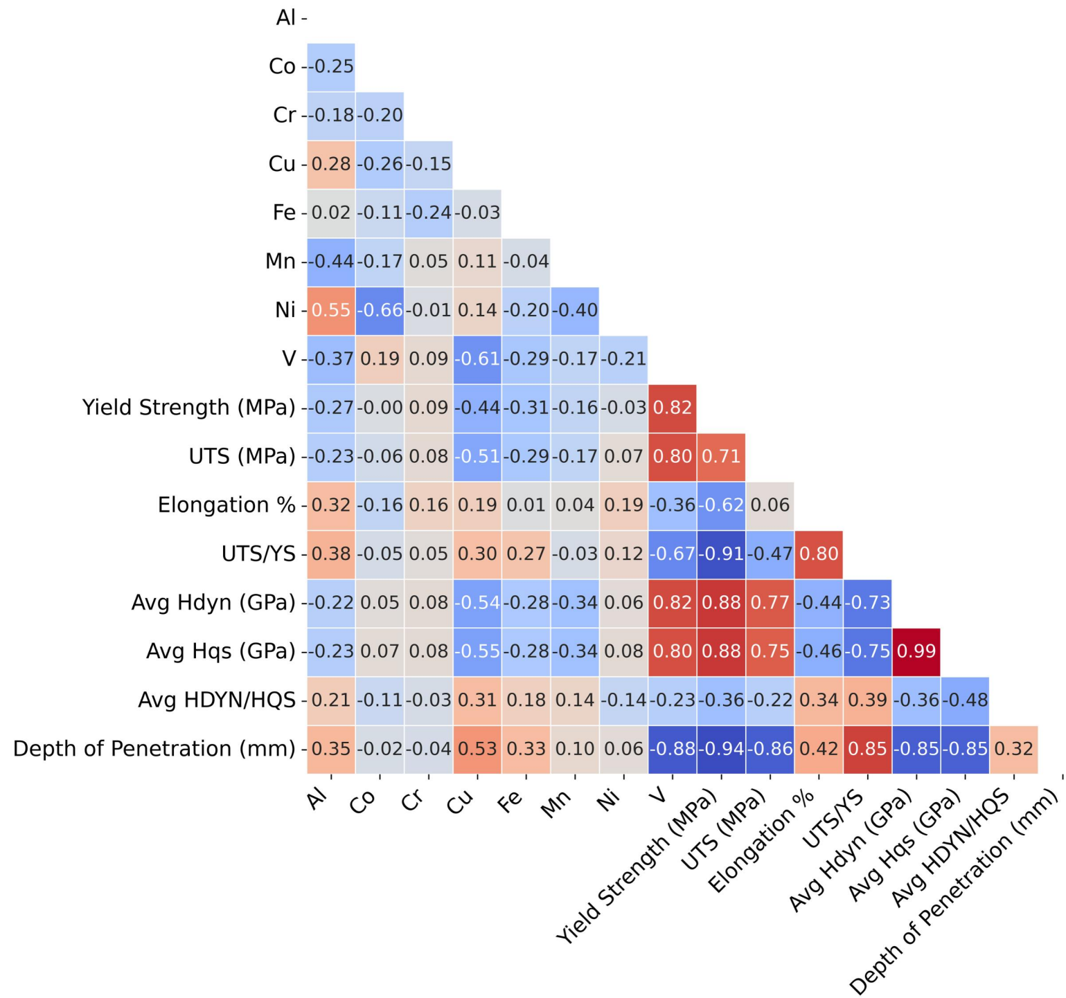
(a) Correlation Matrix
