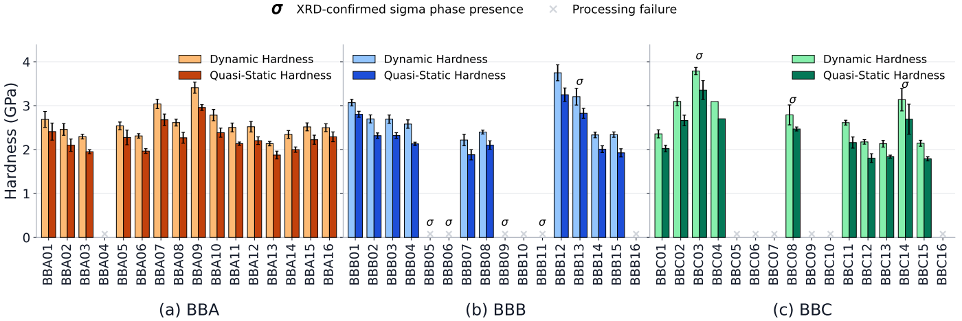
Figure 12. Dynamic and quasistatic hardness values for all candidate alloys across iterations (a) BBA, (b) BBB, and (c) BBC. Bar colors are iteration-specific within each panel. Gray × markers denote processing failures with no hardness data, and \sigma markers indicate alloys with XRD-confirmed sigma phase presence.
