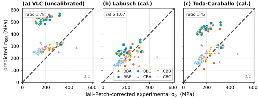
Figure S10: Family 2 SSS estimates versus Family 1 Hall–Petch-corrected YS.
