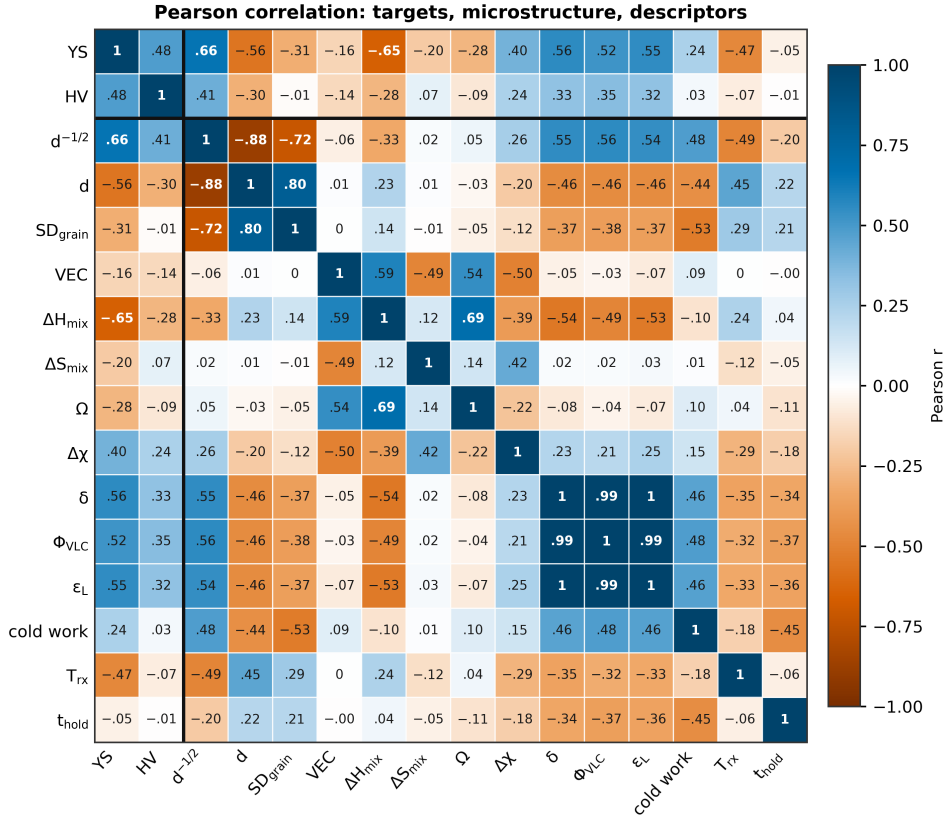
Figure S4: Pearson correlation matrix for composition, processing, grain-size, and descriptor variables. Correlation is descriptive and does not establish independent mechanistic effects.
