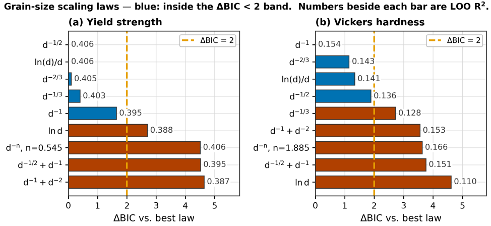
Figure S6: Information-criterion differences among pre-specified YS grain-size laws.
