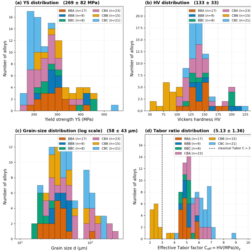
Figure S2: Audited YS, HV, grain-size, and effective hardness-to-yield distributions by batch.
