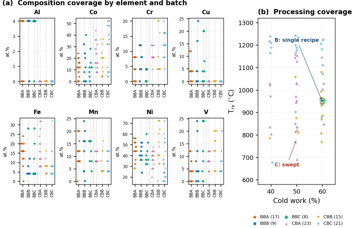
Figure S1: Composition and processing coverage by batch. The B campaign uses one fixed processing condition, while the C campaign spans a processing grid. The coverage follows the experimental design and is not a random sample of the composition simplex.
