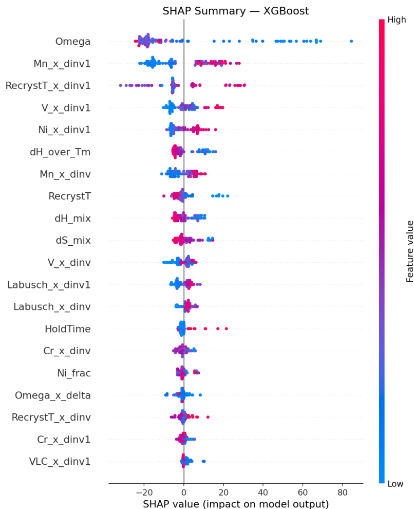
Figure S11: SHAP summary for the archived XGBoost model. The values explain this predictor, which was tuned using the full dataset; they are not causal feature effects.
