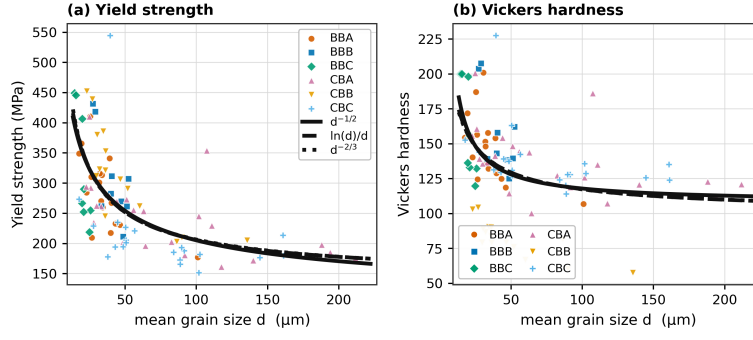
Figure S7: Top Family 1 YS scaling laws over the observed grain-size range. Their close overlap shows why the data do not identify a unique exponent.
