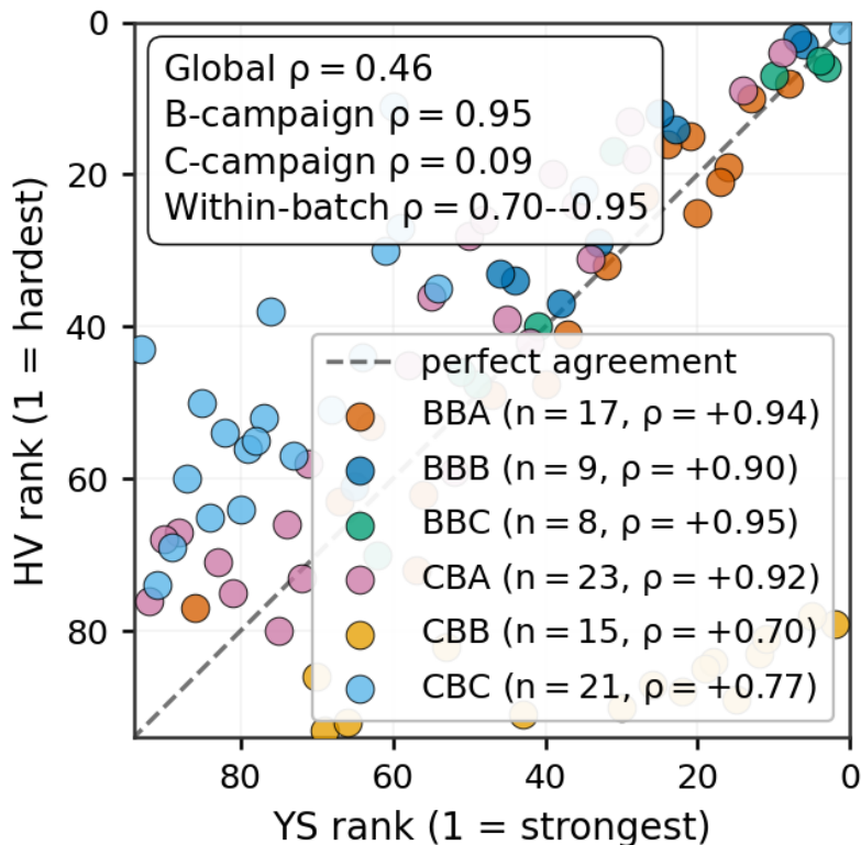
Figure S13: HV rank versus YS rank by batch. Strong ordering within each batch becomes weaker after pooling because composition and processing coverage differ among batches.
