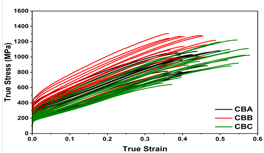
Figure S3: True stress-strain curves for the C-campaign records at a nominal strain rate of 5 \times 10^{-4} \text{ s}^{-1} . The 0.2% offset values are the YS targets used in the analysis.
