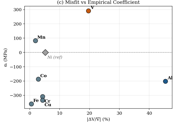
Figure 3: Empirical M3 friction-stress coefficients \alpha_i versus fractional volume misfit |\Delta V_i/V| (Ni reference, \alpha_{\text{Ni}} \equiv 0 ). V’s standout positive coefficient (+291 MPa, \sim 20\% misfit) aligns with the parameter-free Varvenne–Curtin prediction; Al has the largest misfit but a strongly negative empirical \alpha , reflecting its low and narrow concentration range (mean 1.1 at.%).
