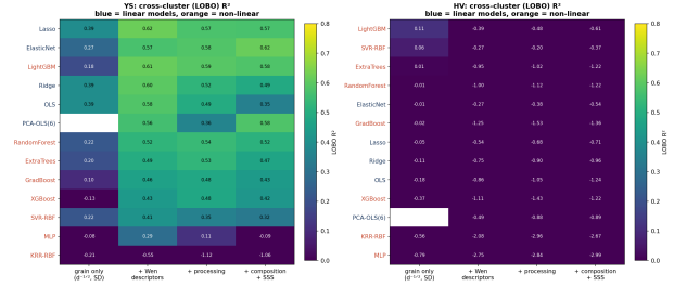
Figure 5: Equal-footing fair comparison: LOBO R^2 across the S1–S4 feature ladder (rows: models at zero-tuning defaults; columns: ladder tiers) for YS and HV. For YS the S1 \rightarrow S2 (+Wen) step, not the model class, produces the lift; for HV every cell is near zero or negative beyond grain-only.
