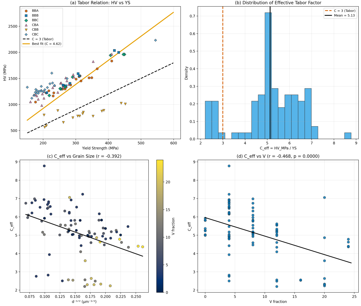
Figure 8: Hardness–yield strength correspondence. (a) HV versus \sigma_y by batch against the classical Tabor line. (b) Distribution of C_{\text{eff}} = \text{HV(MPa)}/\sigma_y (mean 5.13 vs. classical 3). (c) C_{\text{eff}} versus d^{-1/2} ( r = -0.39 ). (d) C_{\text{eff}} versus V fraction ( r = -0.47 ).
