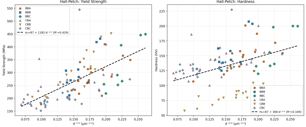
Figure 2: Classical Hall-Petch analysis: yield strength versus d^{-1/2} for the 93 FCC HEAs with tensile data, colored by experimental batch. The global regression (LOO R^2 = 0.406 ) leaves substantial residual variance attributable to composition.
