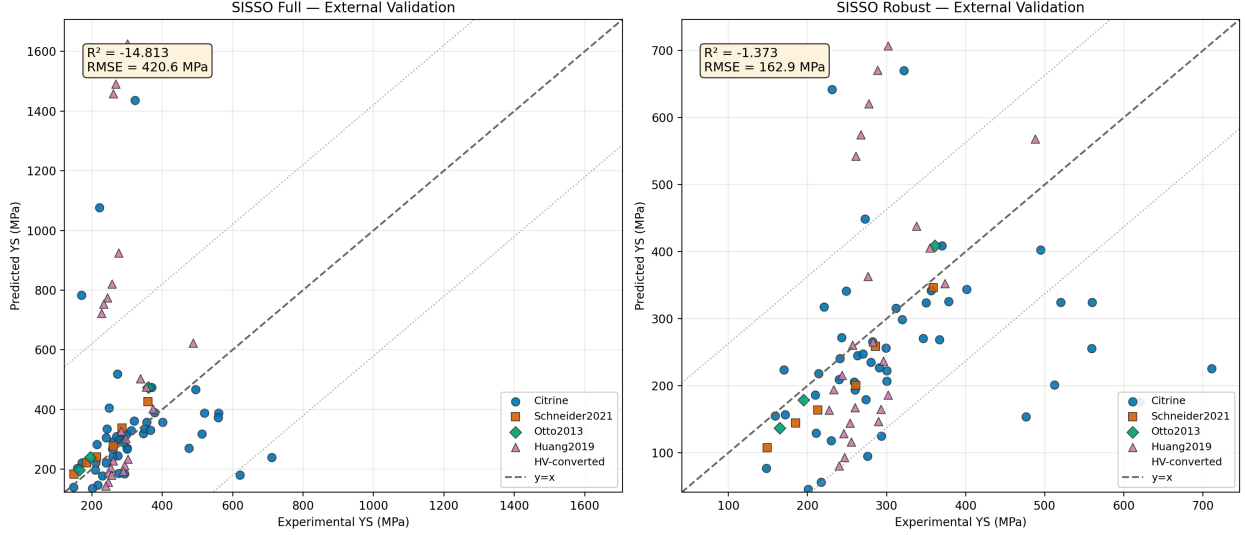
Figure 7: External validation on 82 independent literature points. (Left) SISSO Full (Eq. 2): catastrophic failure ( R^2 = -14.8 , \text{RMSE} = 421 MPa) driven by the \sigma_x^2/\delta_\mu singularity on Mn-containing ternaries. (Right) SISSO Robust (Eq. 3): the pathology disappears ( \text{RMSE} = 163 MPa, bias -32 MPa). M3 (not shown) yields \text{RMSE} = 133 MPa.
