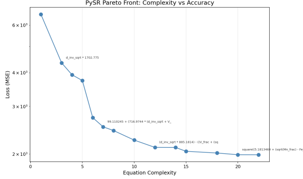
Figure 6: PySR complexity–loss Pareto front for YS on the F3 (curated-Wen) + O3 grid cell. The elbow (parsimonious knee, Eq. 1) and accuracy solutions are marked; marginal gains are exhausted well before the dataset’s noise ceiling.
