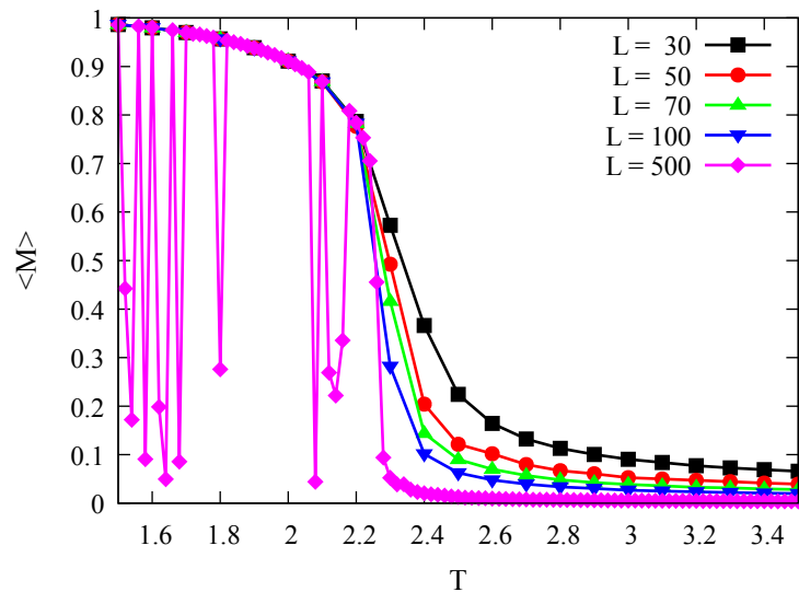
2D Ising Model Results
