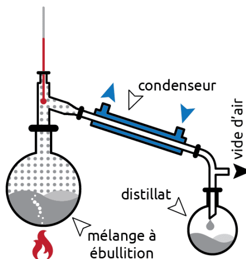
FIGURE 3.8 – Distillation simple
