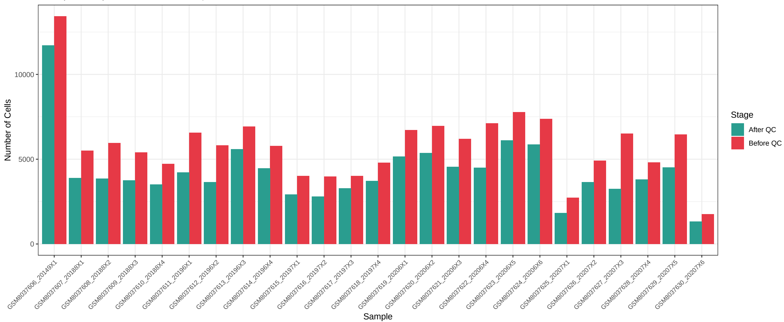
Cells per Sample – Before vs After QC
