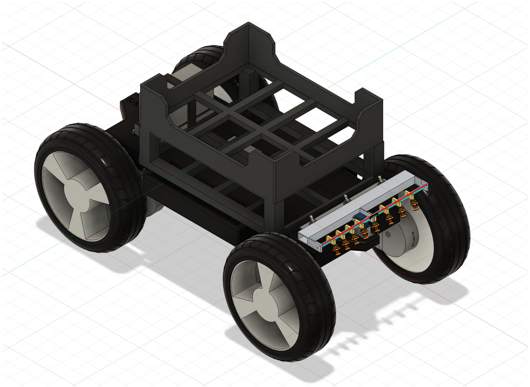
Chassis Without Tank Isometric View
