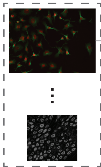
Source Dataset
