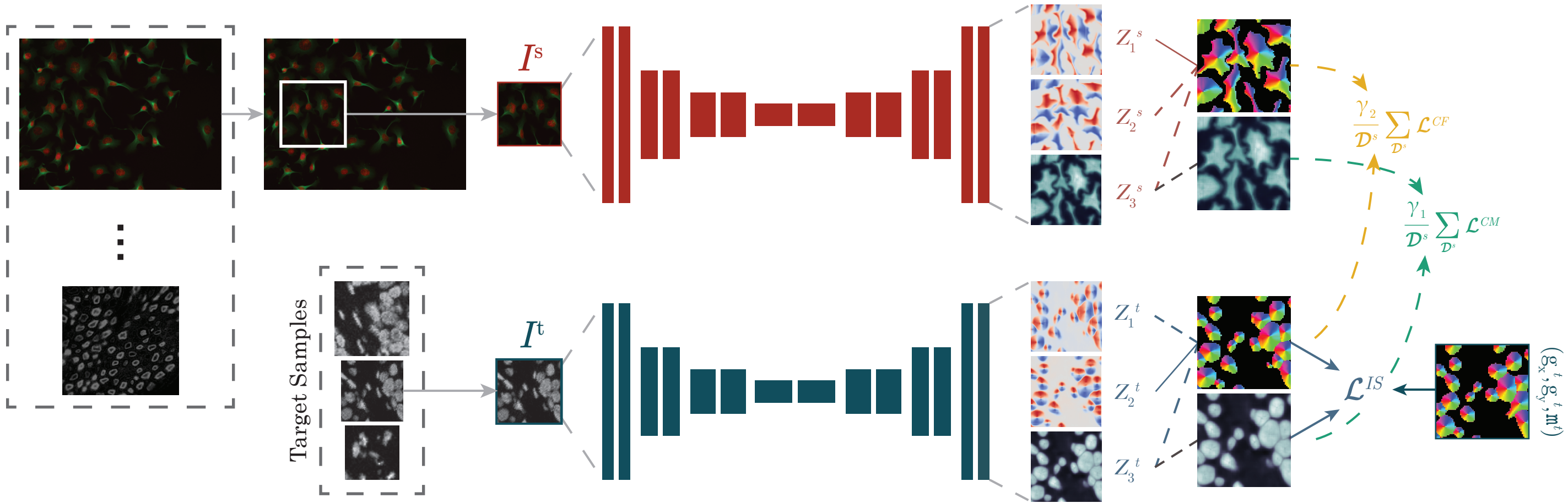
Source Dataset
