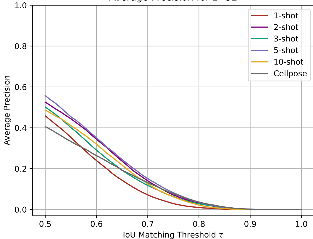
Average Precision for z=32
