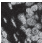
Target Samples
