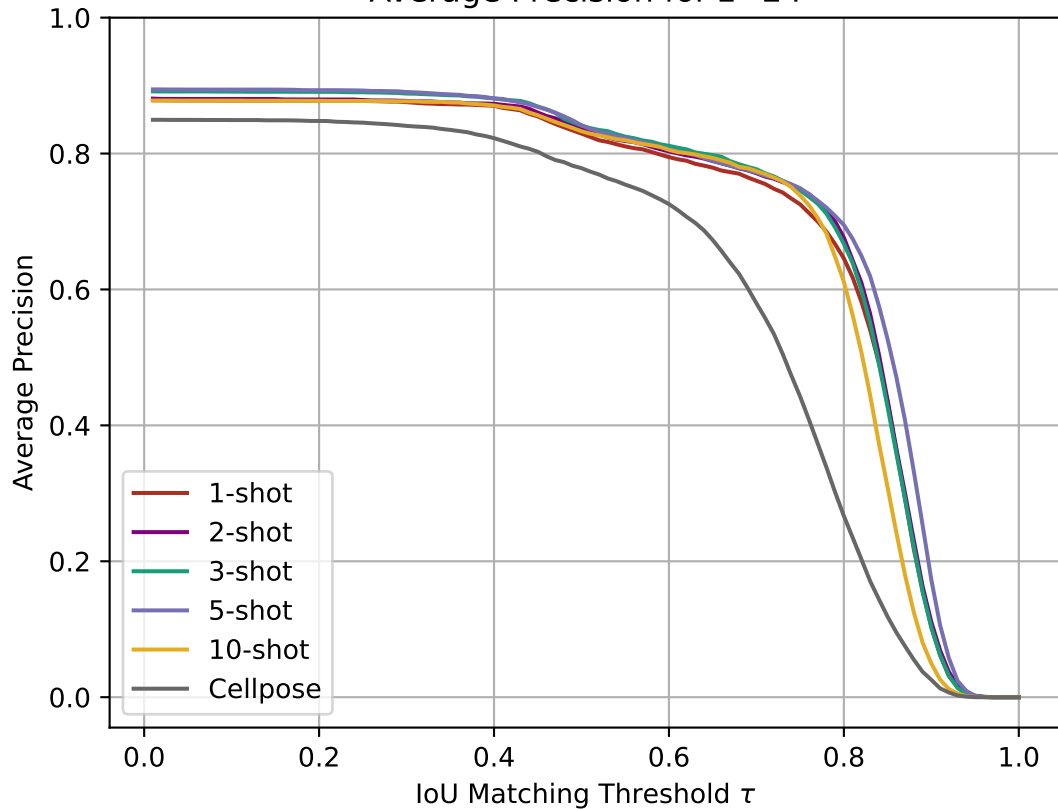
Average Precision for z=24
