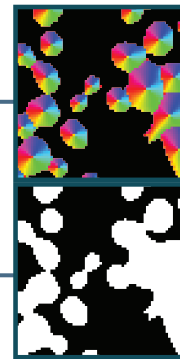
Target Labels
