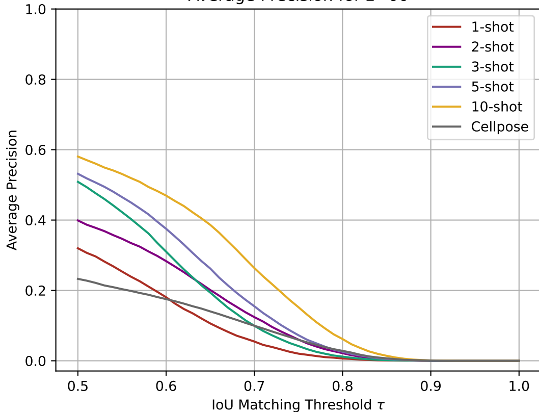
Average Precision for z=00
