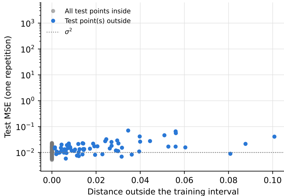
Degree 10
