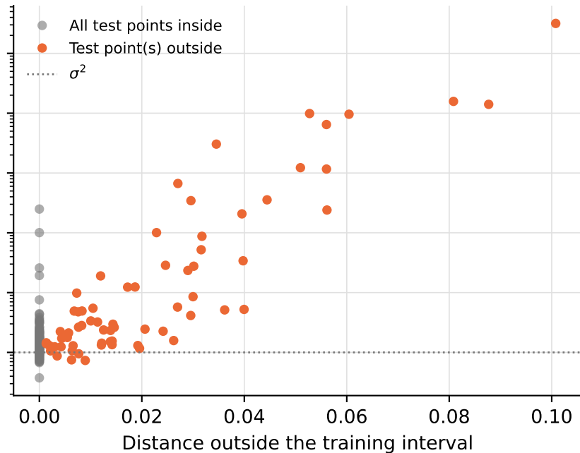
Degree 20
