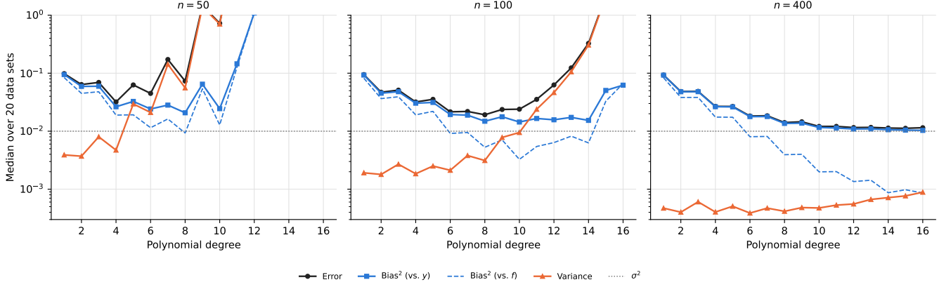
FIG. 9. Bootstrap estimates of the test error, squared bias and variance against degree for OLS, n = 50, 100 and 400 , \sigma = 0.1 , 100 bootstrap samples; median over 20 data sets. Solid bias: measured against y ; dashed: against the true f . Dotted line: \sigma^2 .
