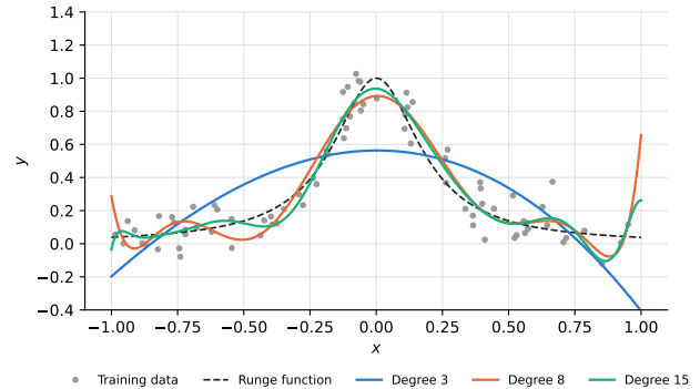
FIG. 17. Training data for seed 42, Runge’s function, and OLS fits of degree 3, 8 and 15. The last training point is at x = 0.951 ; beyond it the degree-8 fit rises to 0.655 at x = 1 , where f(1) = 0.038 .
