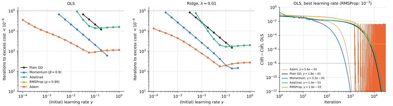
FIG. 13. Degree 6, seed 42, start at \theta = 0 . Left and middle: iterations until the cost is within 10^{-8} of the closed-form minimum against the (initial) learning rate, for OLS and Ridge ( \lambda = 10^{-2} ); missing points did not reach it within 10^5 iterations (RMSProp never does). Right: excess cost against iteration for OLS at each method’s best learning rate (RMSProp at 10^{-3} ), first 3 \times 10^4 iterations.
