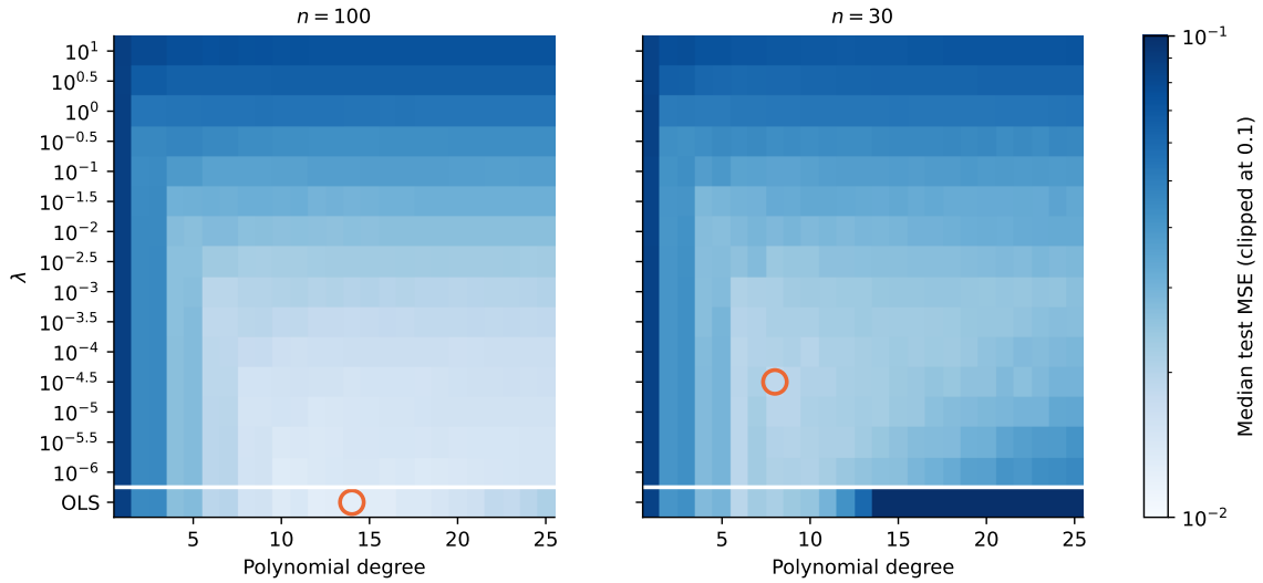
FIG. 6. Median test MSE over 200 repetitions against degree and penalty, n = 100 (left) and n = 30 (right), \sigma = 0.1 . The bottom row is OLS. Colours are clipped at 0.1. Circle: the lowest median.
