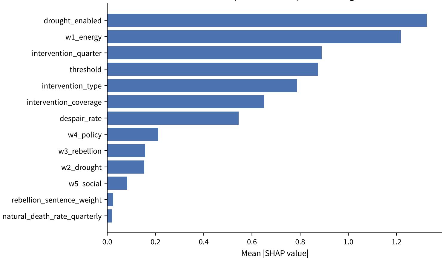
SHAP feature importance — importance_regression
