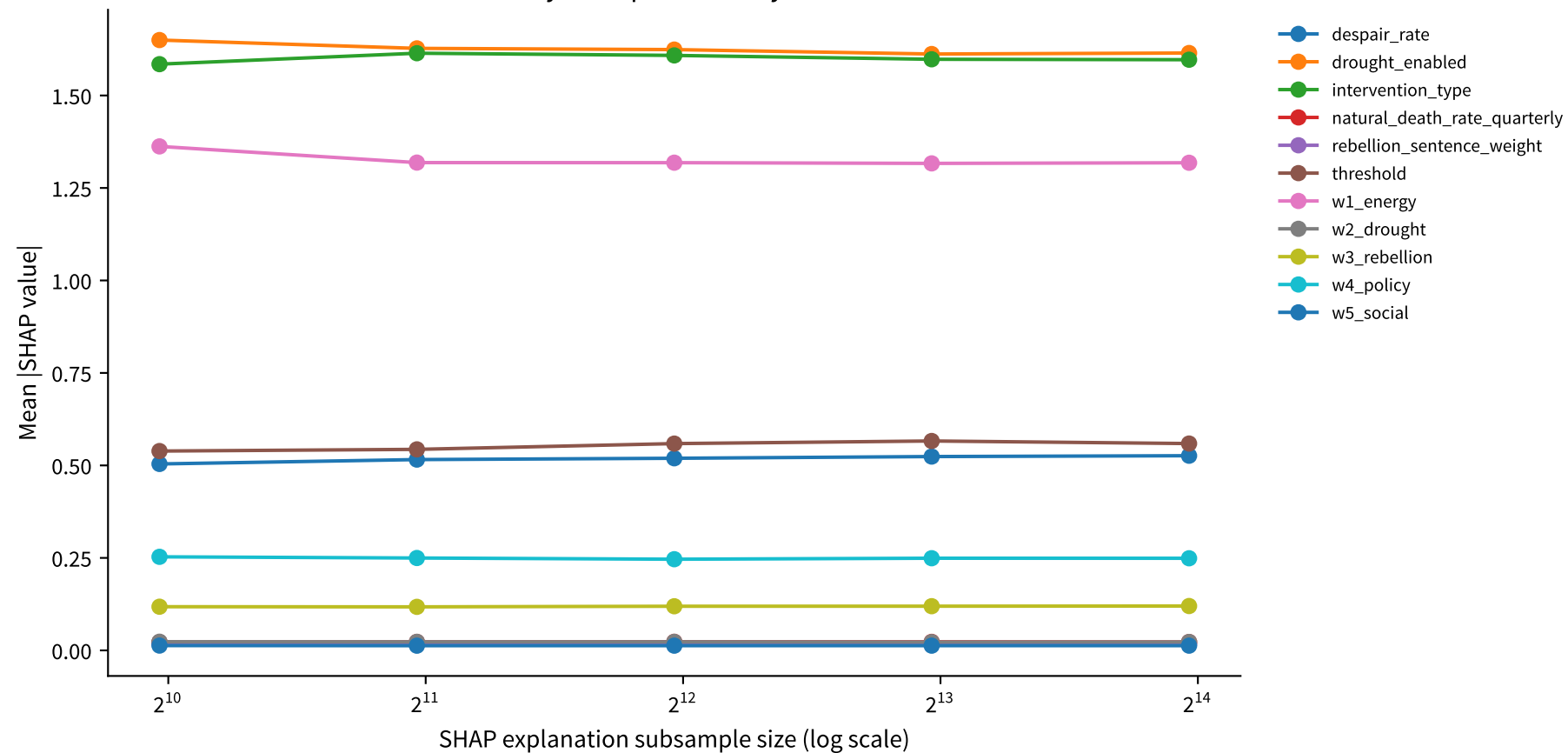
SHAP stability sweep — stability_classification
