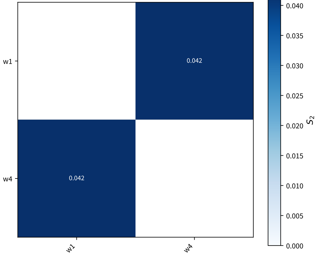
Second-order interactions ( S_2 ) — peak_mutiny
