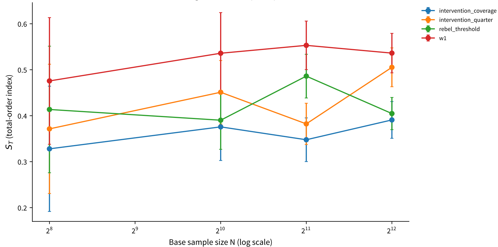
Sobol convergence — collapse_quarter
