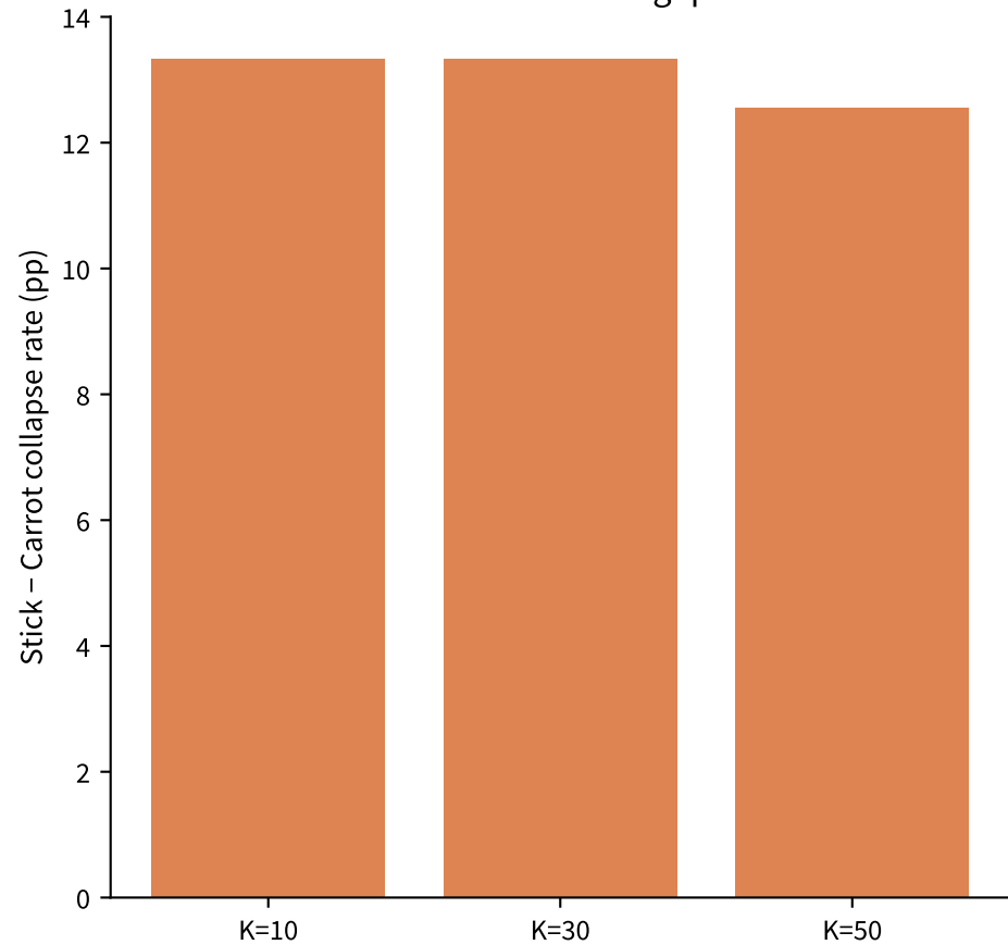
Carrot vs. Stick gap
