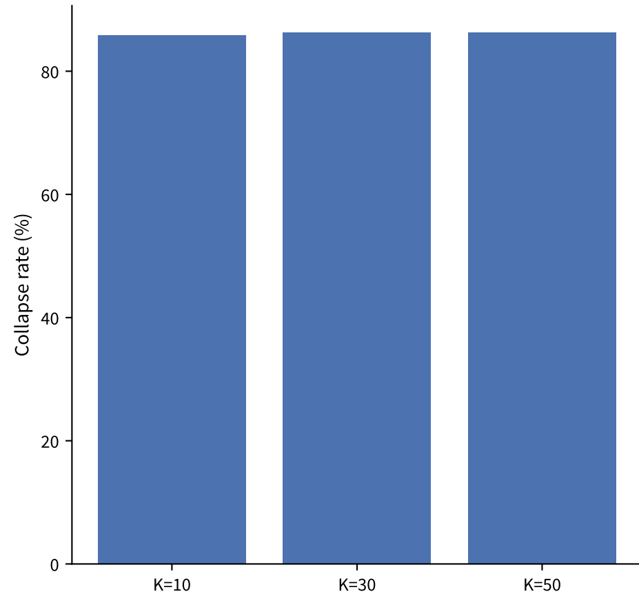
Overall collapse rate
