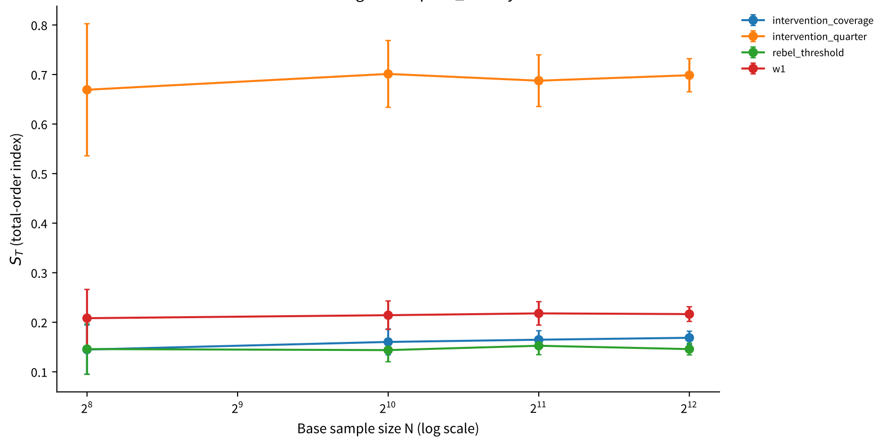
Sobol convergence — peak_mutiny
