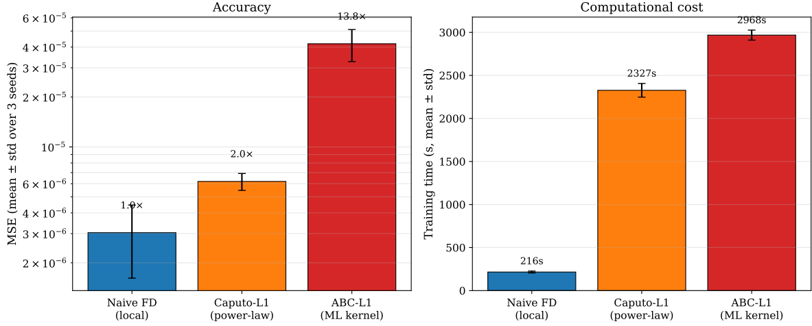
Figure 8: Accuracy–cost trade-off across the three residuals. Left: MSE (mean \pm std over 3 seeds, log scale). Right: training time. The price of genuine non-locality is quantified: Caputo-L1 is 2.0 \times worse in MSE at 10.8 \times the cost; ABC-L1 is 13.8 \times worse at 13.8 \times the cost.
