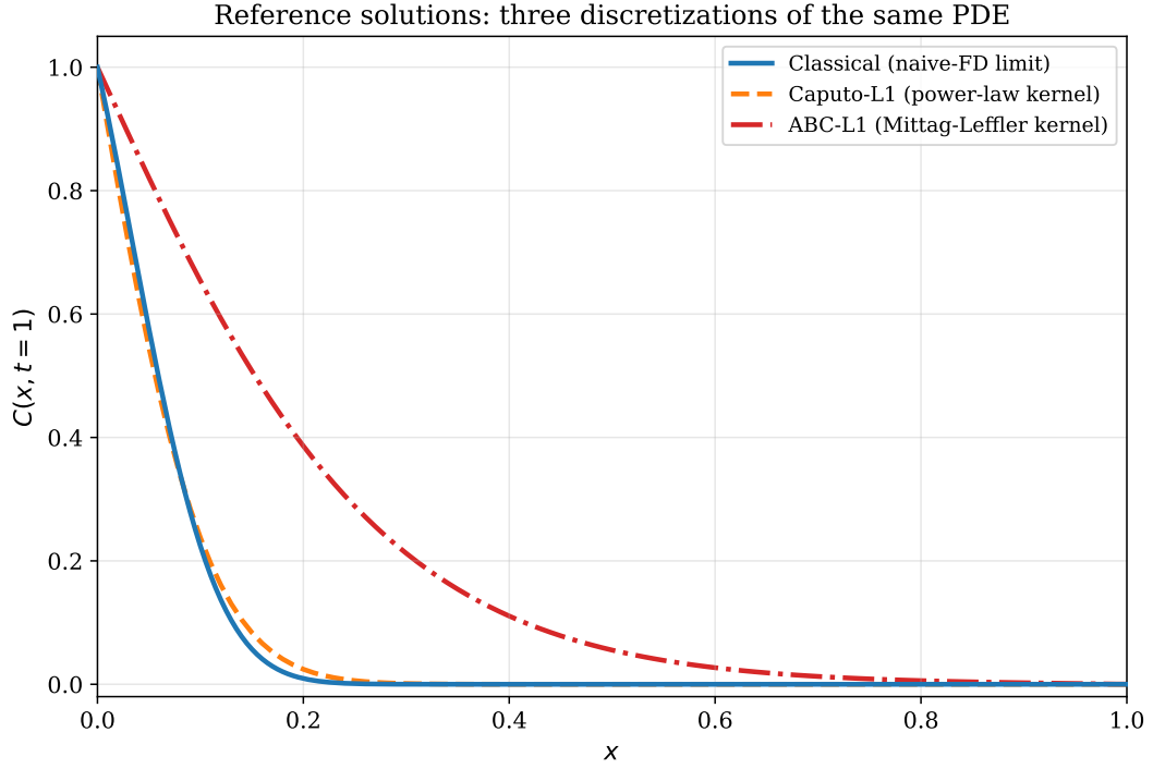
Figure 2: Reference solutions at t = T = 1 for the three discretizations of the same PDE: the classical limit (solid), Caputo-L1 with power-law kernel (dashed), and ABC-L1 with Mittag-Leffler kernel (dash-dot). The three profiles differ substantially, confirming that the three residuals are not interchangeable.
