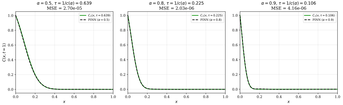
Figure 7: Test 3 (effective-time) applied to the naive-FD PINN for \alpha \in \{0.5, 0.8, 0.9\} . Solid green: base solution C_1(x, \tau) at the effective time \tau = 1/c(\alpha) . Black dashed: PINN prediction at t = 1 . The two profiles coincide within training error, confirming that the naive-FD PINN samples the classical solution at the rescaled time \tau = T/c(\alpha) .
