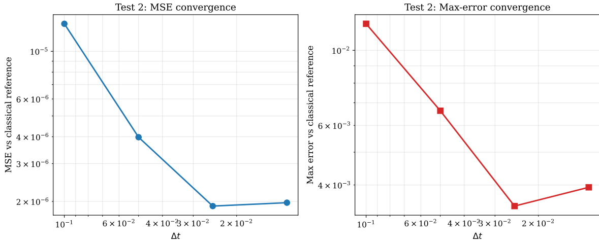
Figure 6: Test 2 ( \Delta t -refinement) applied to the naive-FD PINN. Left: MSE versus \Delta t (log-log). Right: maximum error versus \Delta t . Both quantities decrease monotonically as \Delta t is reduced, before saturating at the PINN’s training-error floor near \Delta t = 0.025 .
