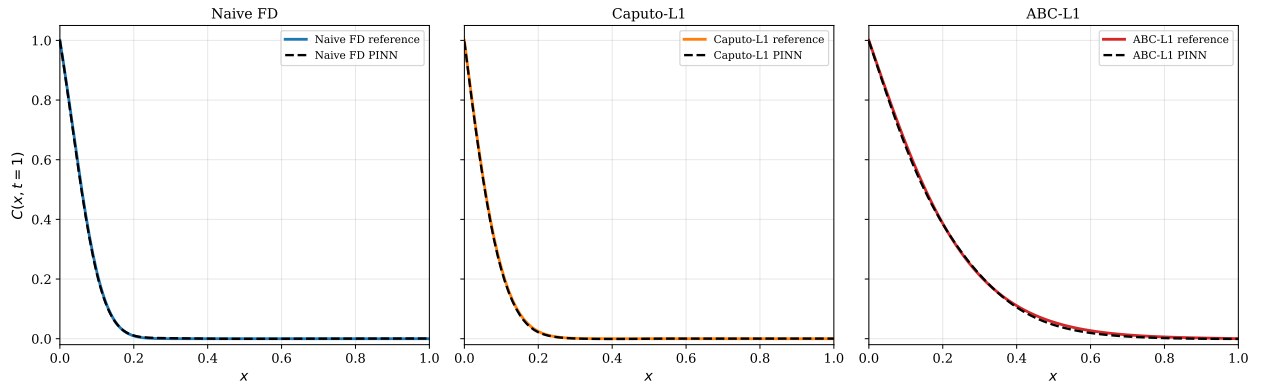
Figure 4: PINN prediction (black dashed) versus reference solution (colored solid) at t = 1 for each of the three residuals. Left: naive FD (local). Middle: Caputo-L1 (power-law). Right: ABC-L1 (Mittag-Leffler). All three PINNs reproduce the qualitative shape of their respective reference, but the quantitative agreement degrades with operator complexity.
