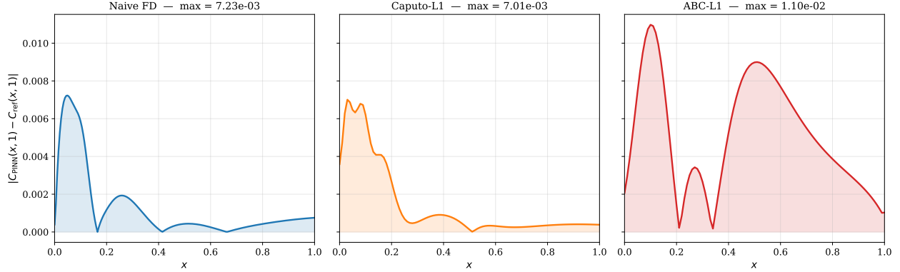
Figure 5: Pointwise absolute error profiles |C_{\text{PINN}}(x, 1) - C_{\text{ref}}(x, 1)| for the three residuals. Shown for seed 42 (representative). The mean maximum errors across three seeds (42, 123, 7) are 7.23 \times 10^{-3} (naive FD), 7.01 \times 10^{-3} (Caputo-L1), and 1.10 \times 10^{-2} (ABC-L1).
