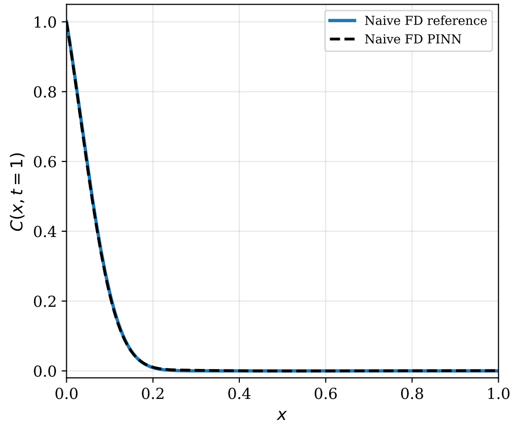
Naive FD
