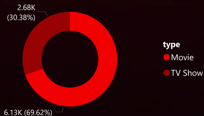
TV Show & Movie
