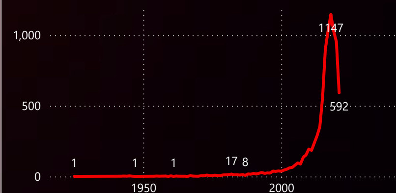
Country Count by Release Year
