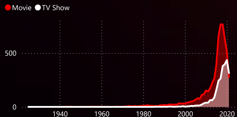
Total Shows by Released Year
