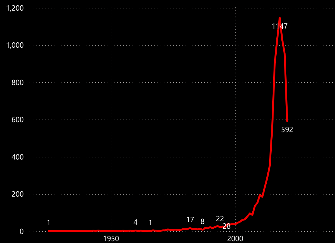
Country Count by Release Year
