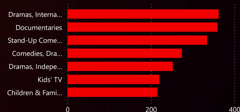
Listed by Total Shows
