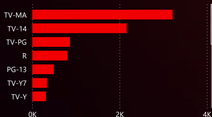
Rating based on Total Shows
