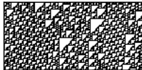
rule 110 (complex)
