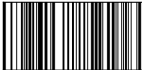
rule 204 (frozen)
