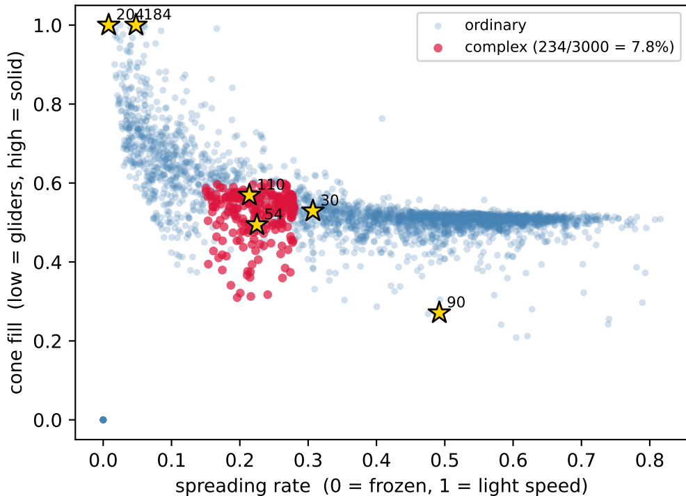
Range-2 behaviour landscape (stars: embedded ECAs)
