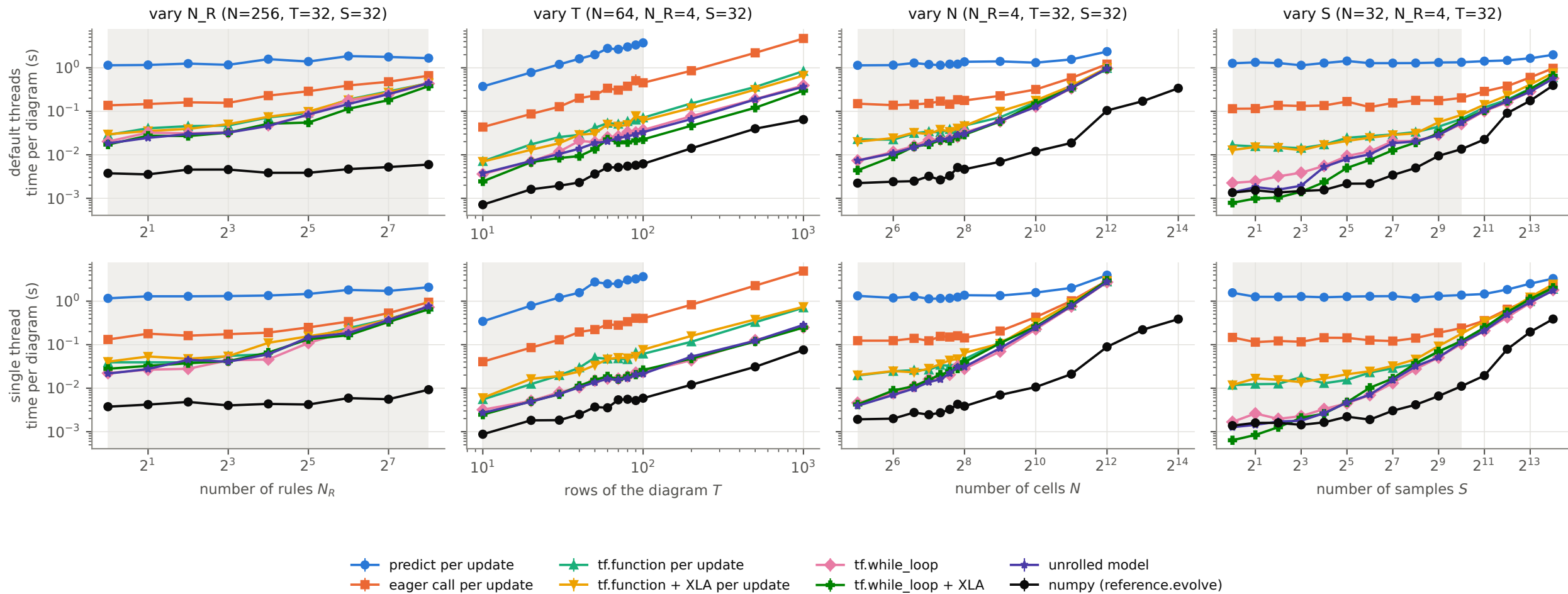
Drivers of the CNN with the dense selector (shaded: range of thesis Tab. 7.2; error bars: interquartile range)
