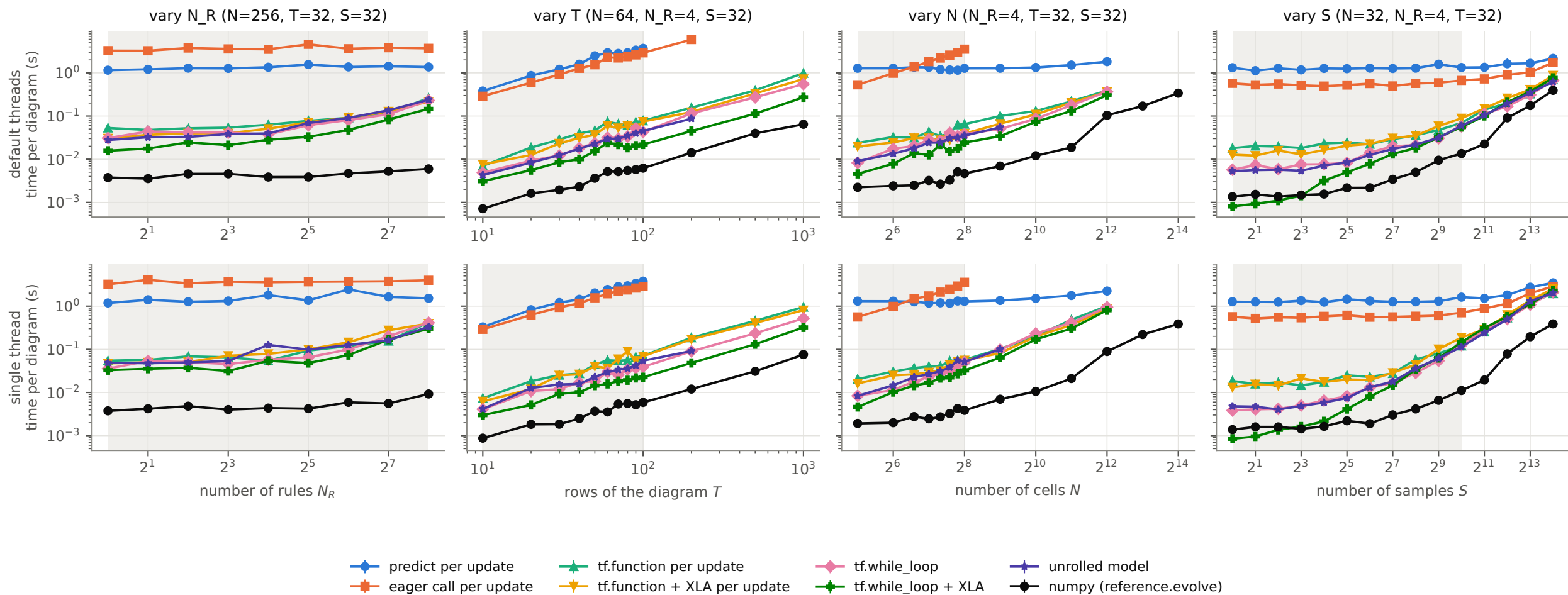
Drivers of the CNN with the LocallyConnected1D (impl. 1) selector (shaded: range of thesis Tab. 7.2; error bars: interquartile range)
