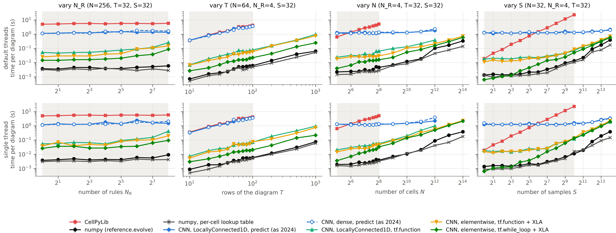
Exact nuCA simulation: overview (shaded: range of thesis Tab. 7.2; error bars: interquartile range)
