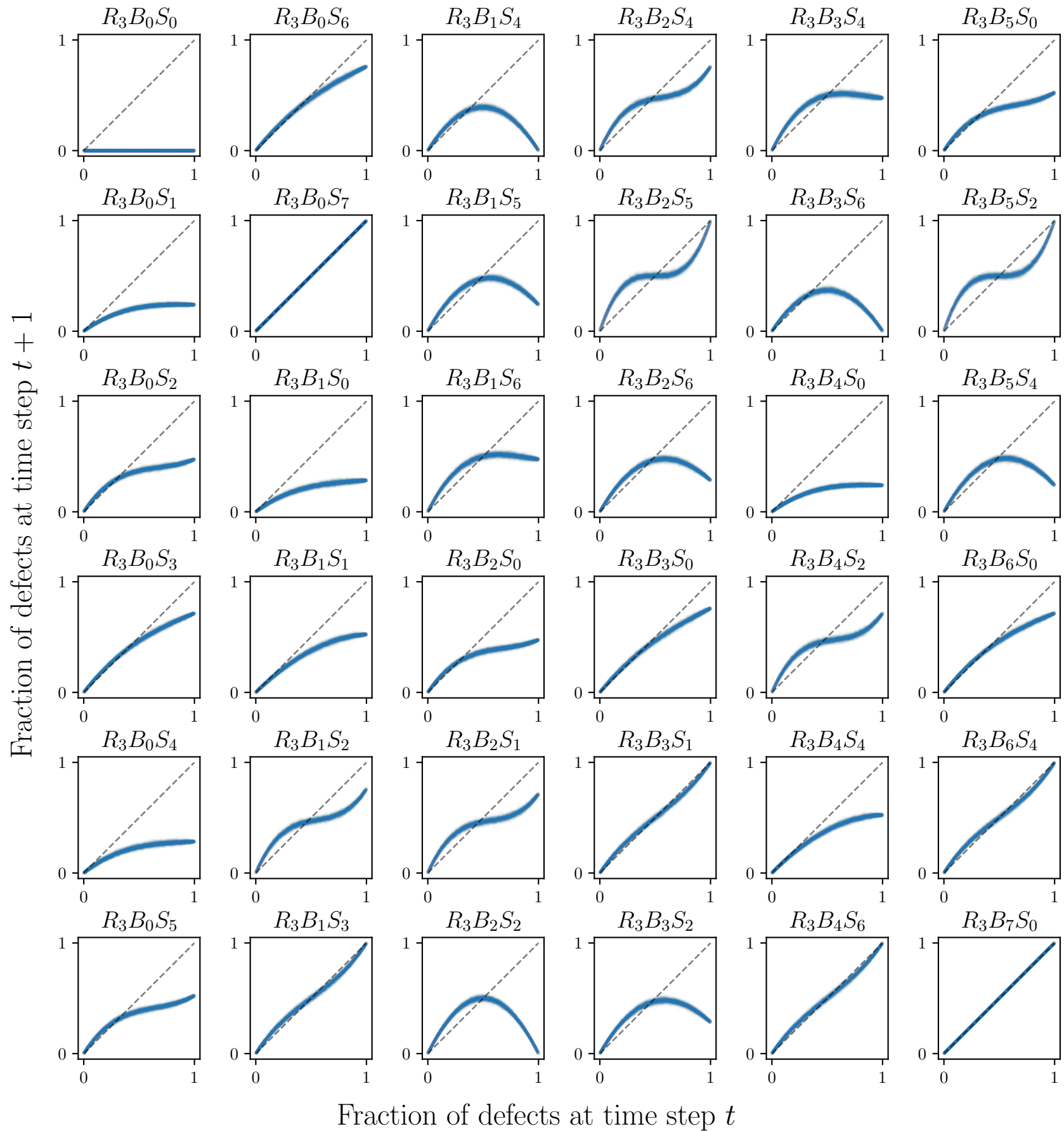
Derrida plots for all nonequivalent resolution-3 LLNAs on a N=1001 ring network
