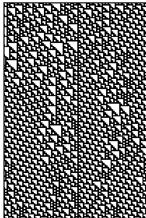
Rule 124
