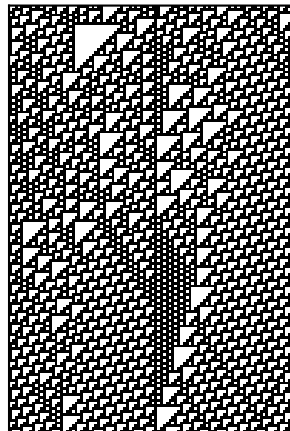
Rule 110
