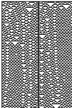
Rule 54
