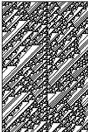
Rule 106
