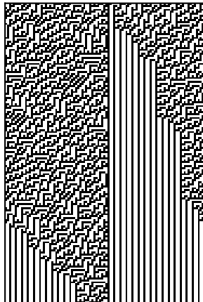
Rule 45
