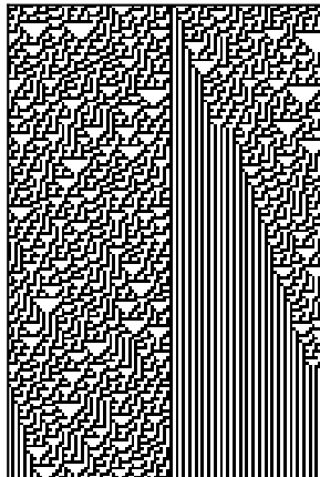
Rule 30
