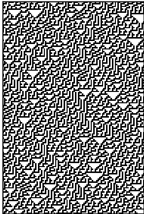
Rule 30, \nu = 0.00
