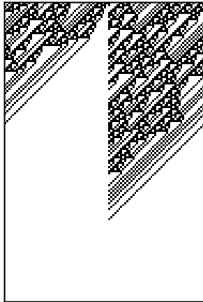
Rule 106, \nu = 0.01
