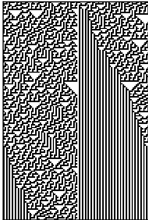
Rule 30, \nu = 0.01
