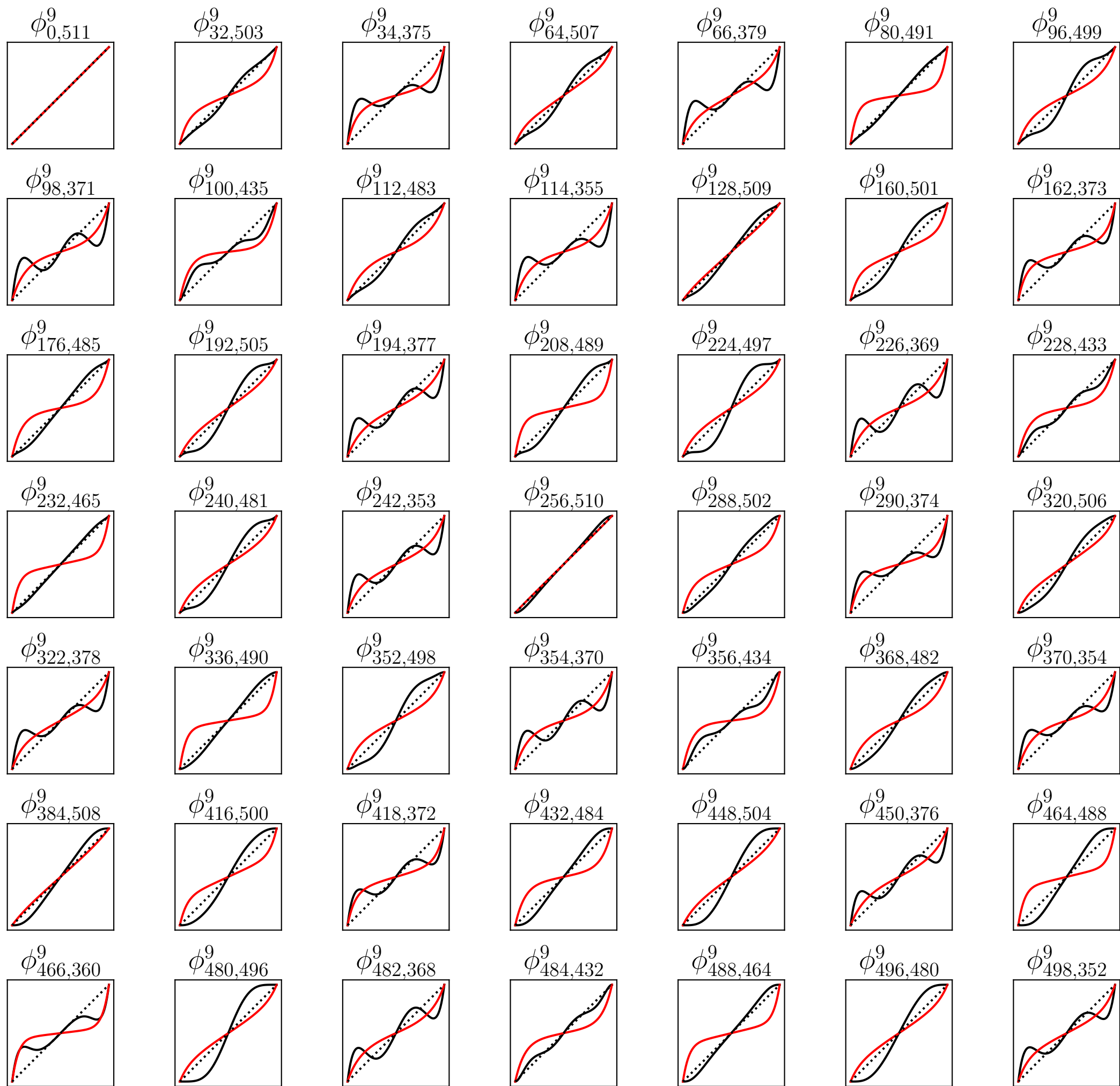
Mean field curves and Derrida curves for all unstable legal self-equivalent LLNA rules of resolution 9, for degree 8
