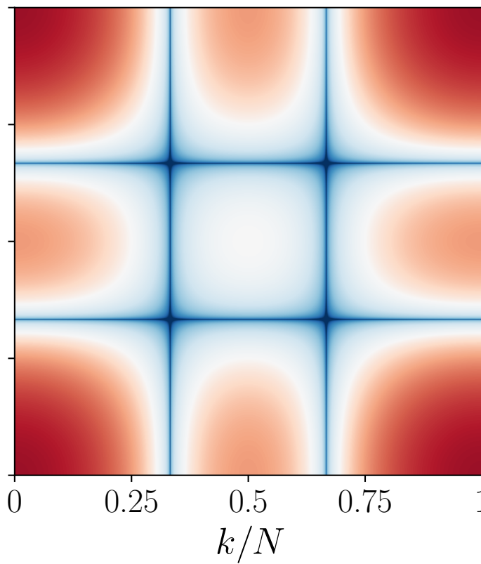
Moore MLE = \ln 9
