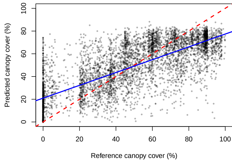
Random Forest
