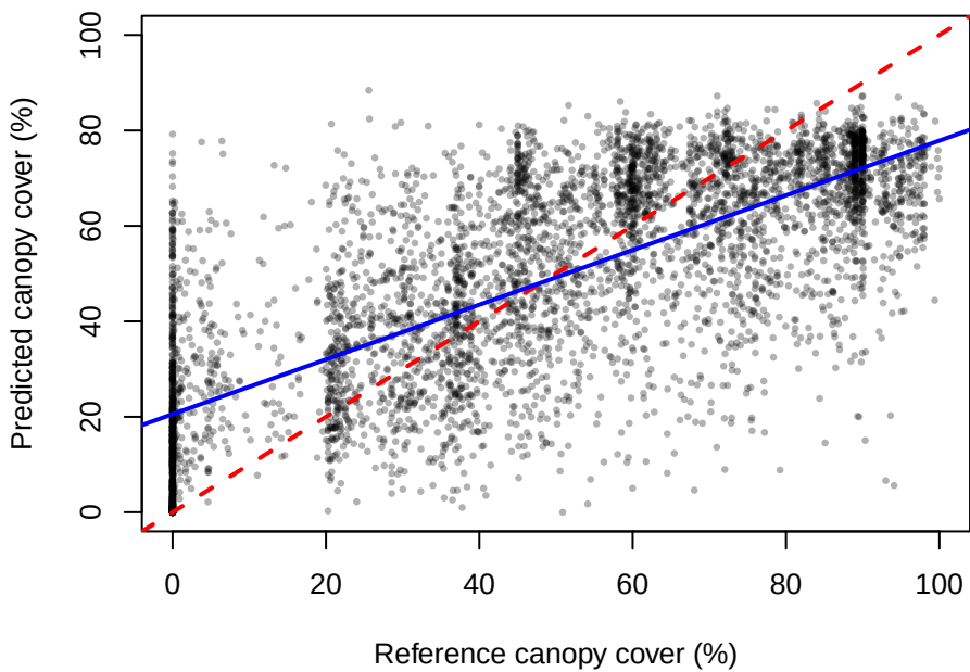
Gradient boosting
