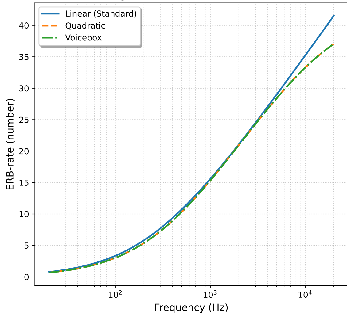
Comparison of ERB-rate scales
