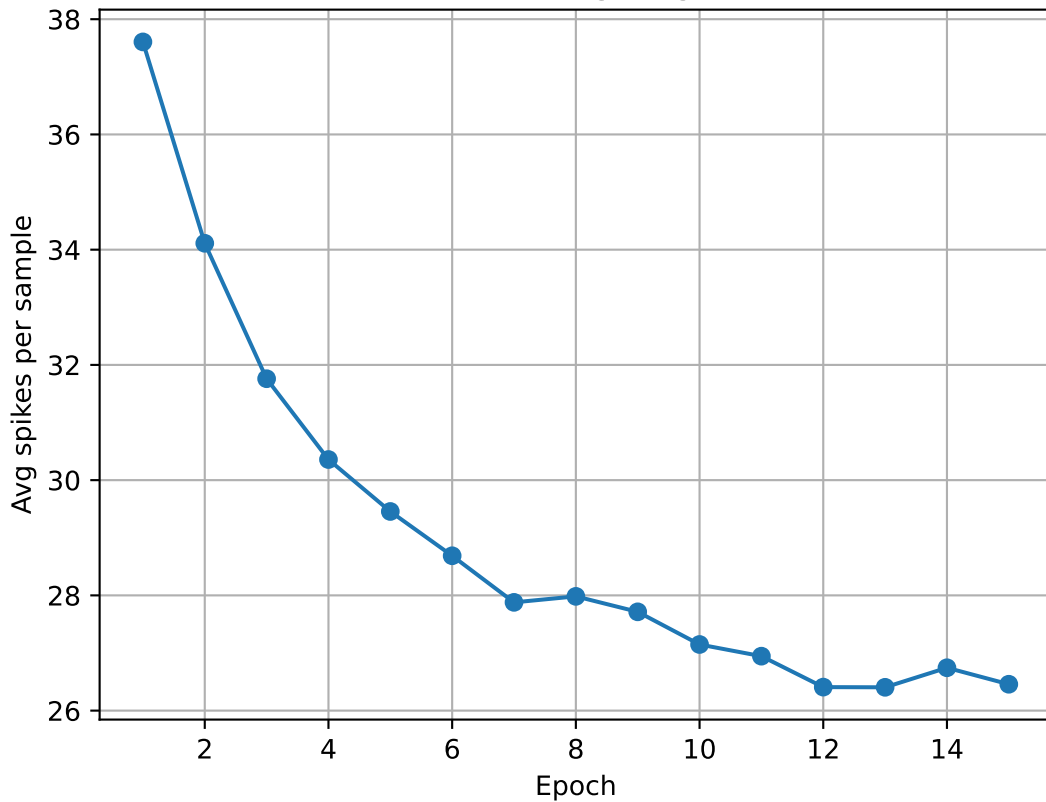
STDP Training Progress
