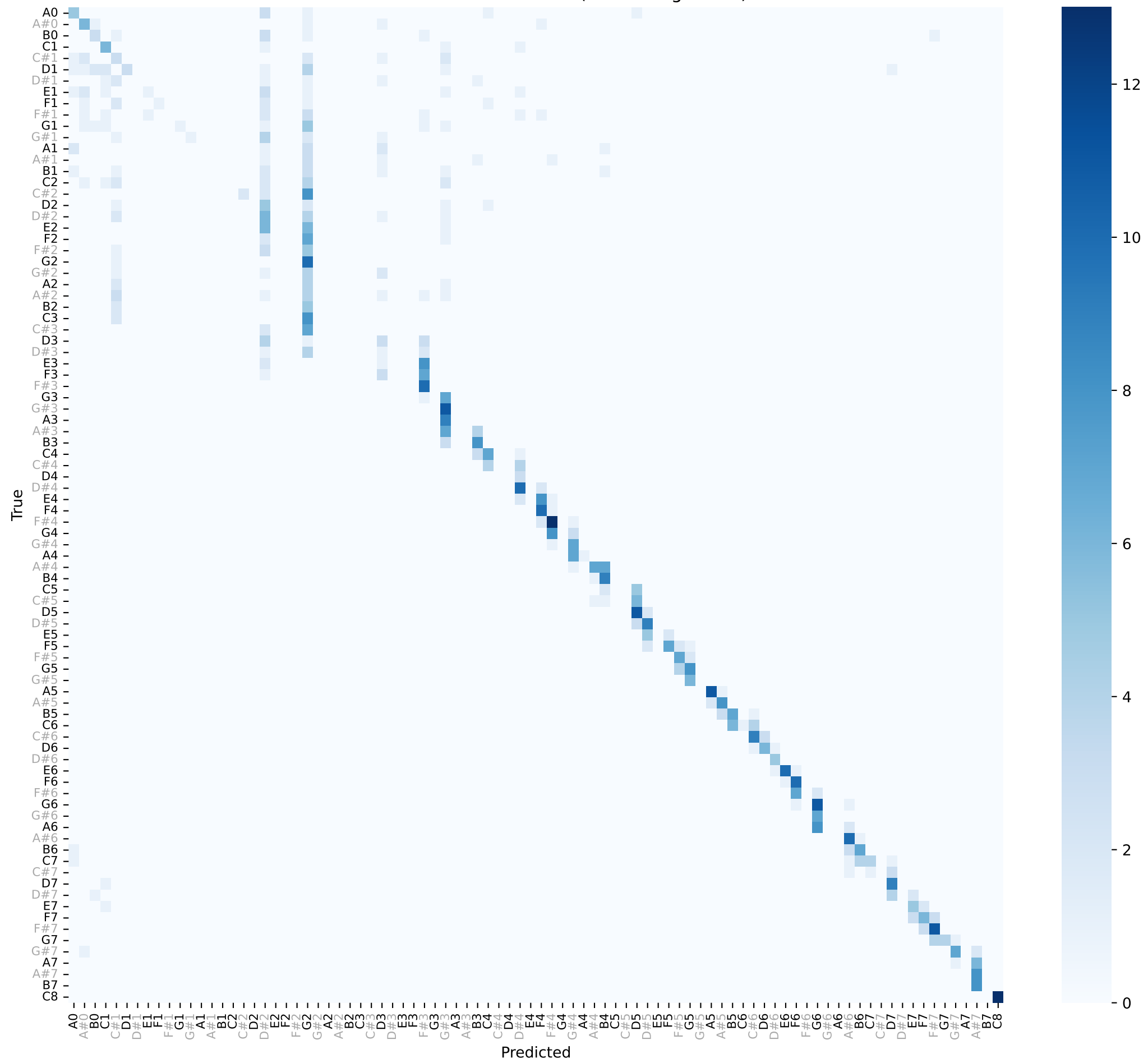
STDP-WTA Confusion Matrix (After Assignment)
