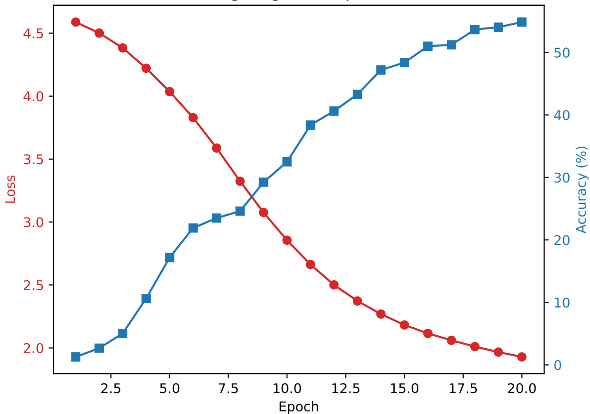
Training Progress (Supervised)
