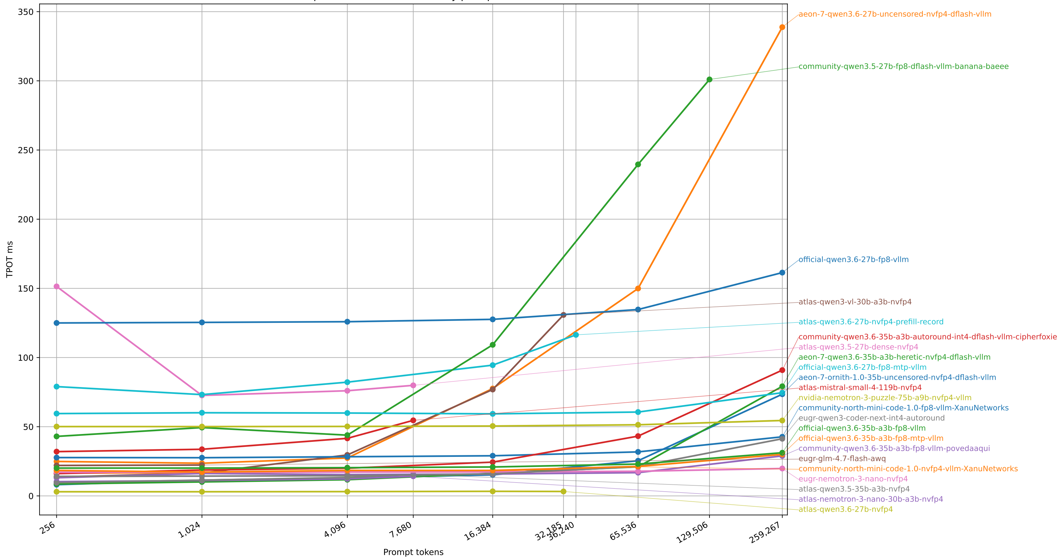
Sparkrun benchmark TPOT by prompt size
