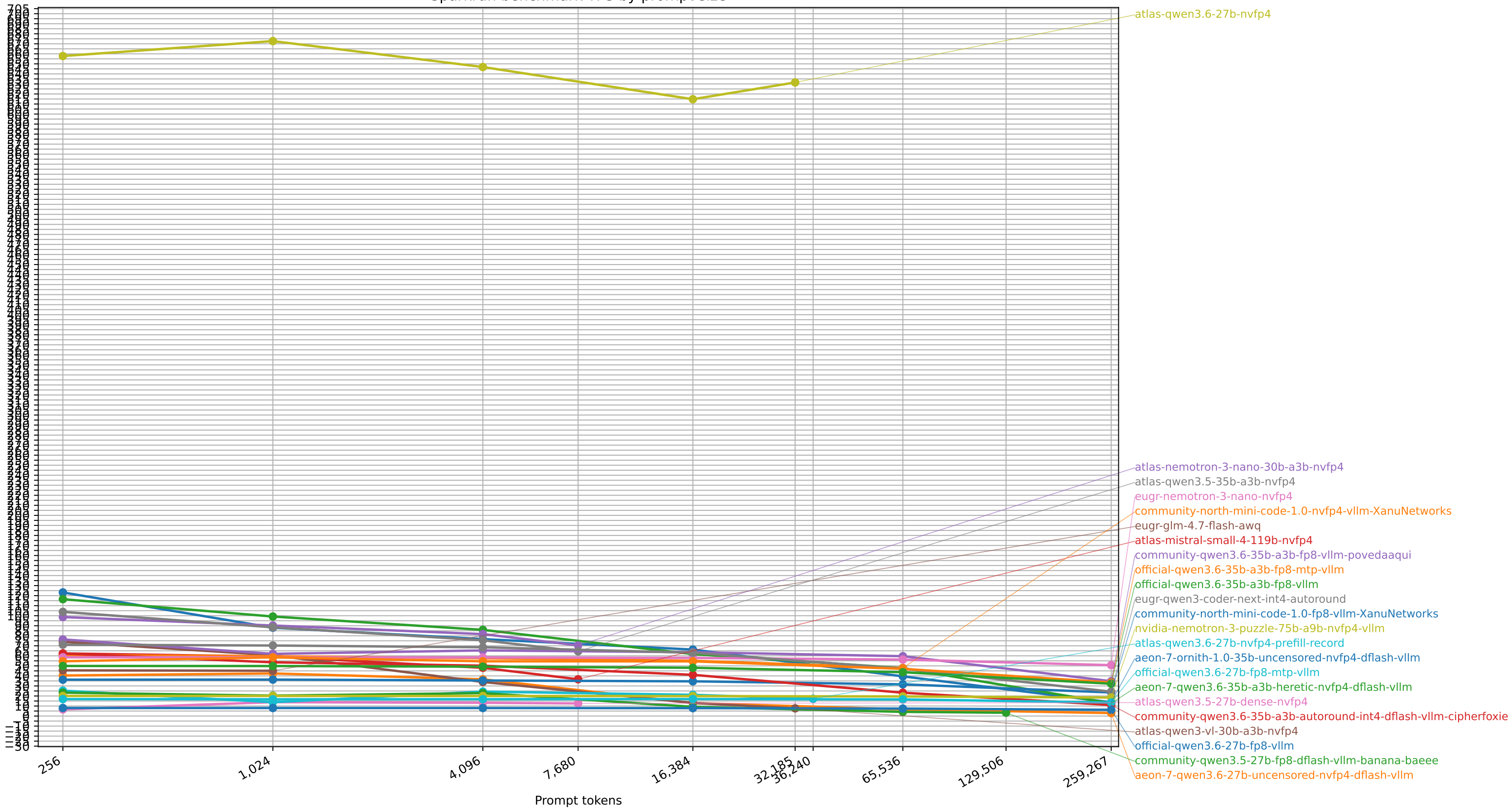
Sparkrun benchmark TPS by prompt size
