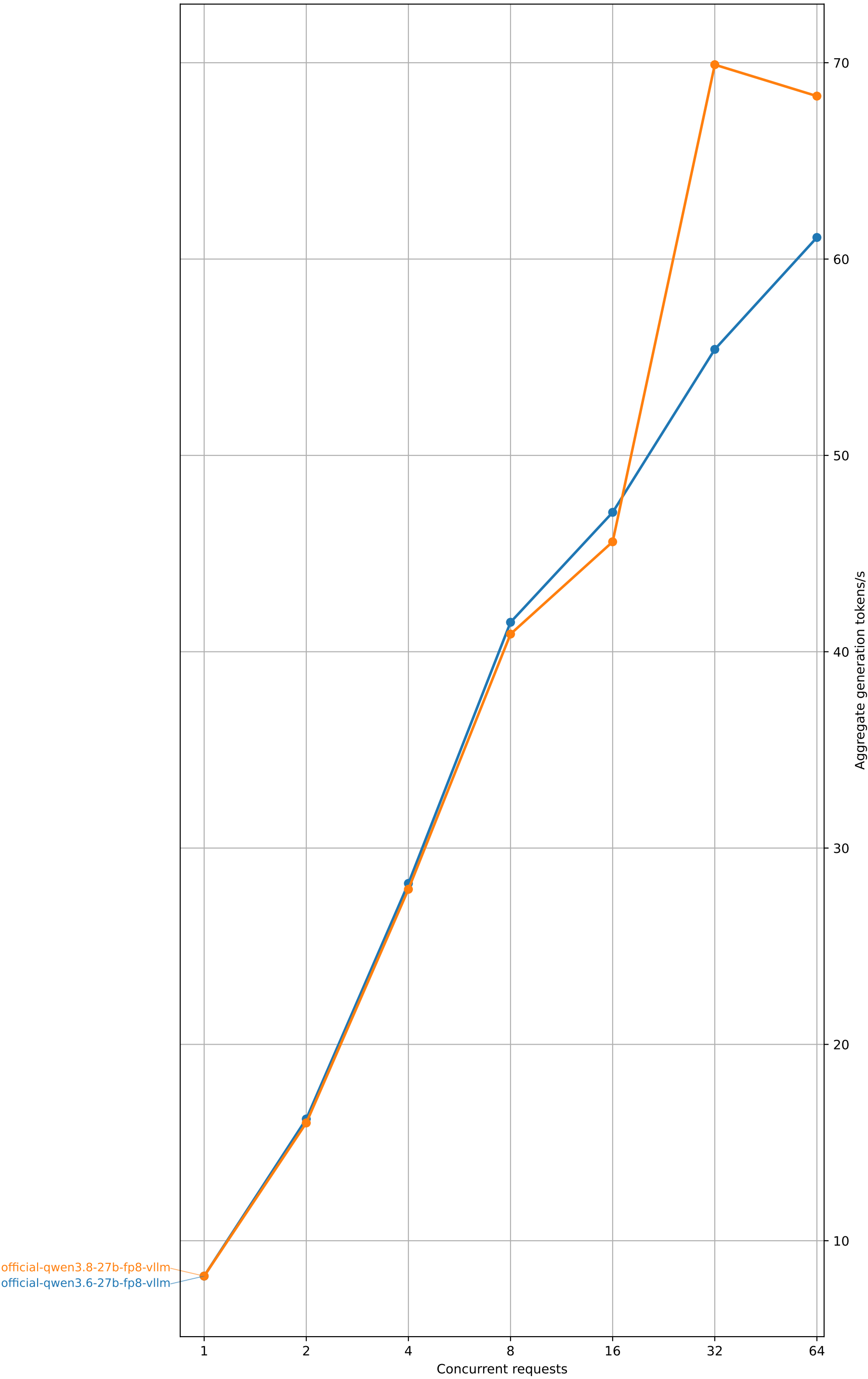
Sparkrun benchmark aggregate TPS by concurrency (1024-token prompts)
