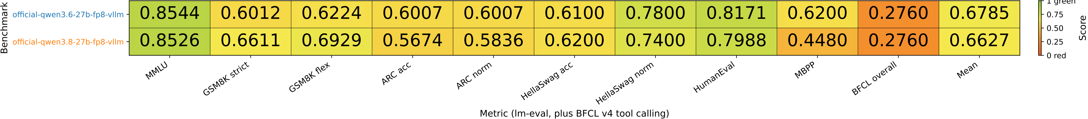
Sparkrun intelligence scores (grey = test failed or could not run)
