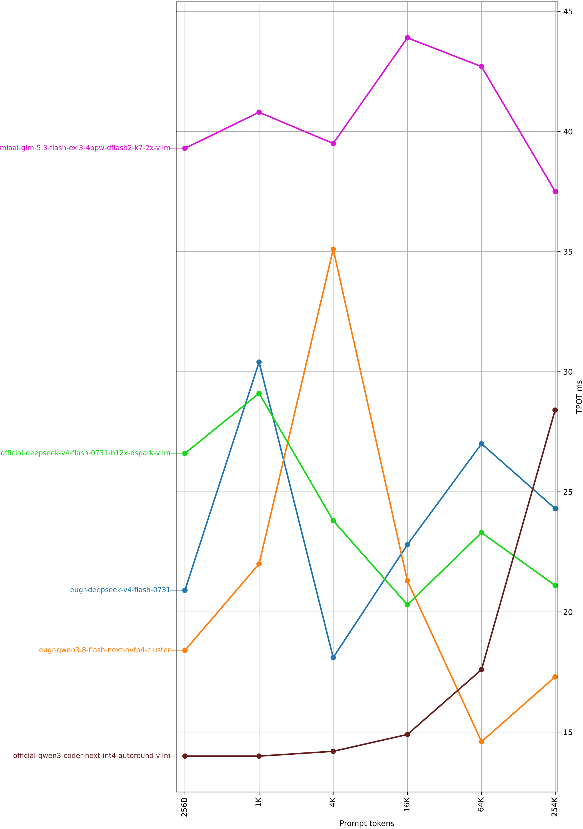
Sparkrun benchmark TPOT by prompt size
