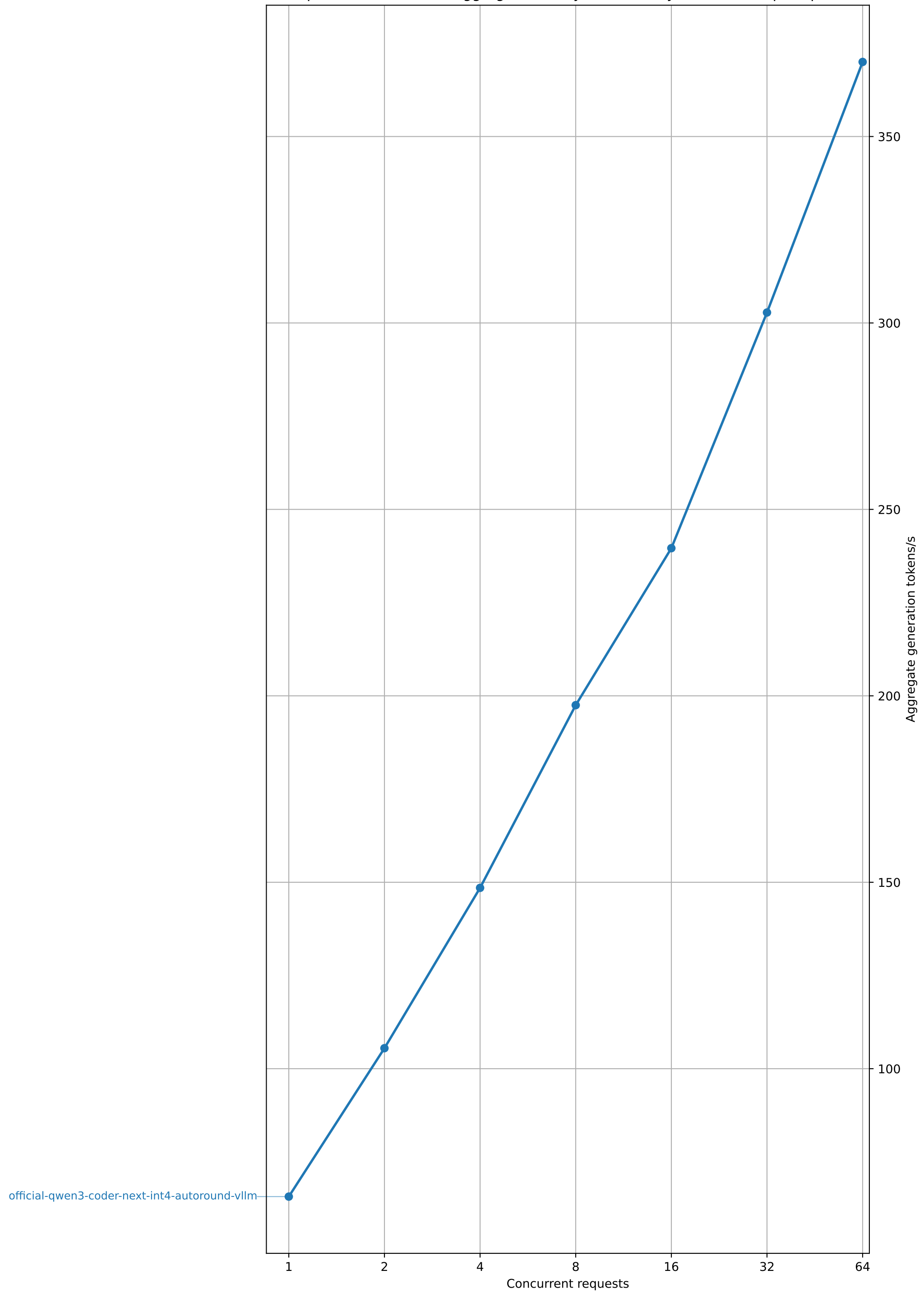
Sparkrun benchmark aggregate TPS by concurrency (1024-token prompts)
