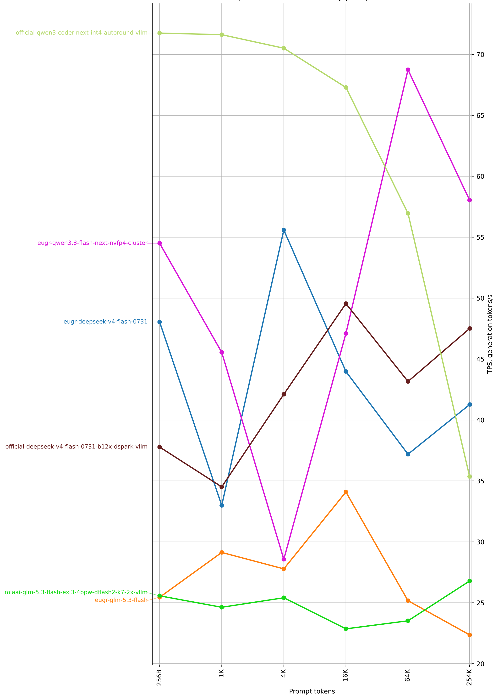
Sparkrun benchmark TPS by prompt size
