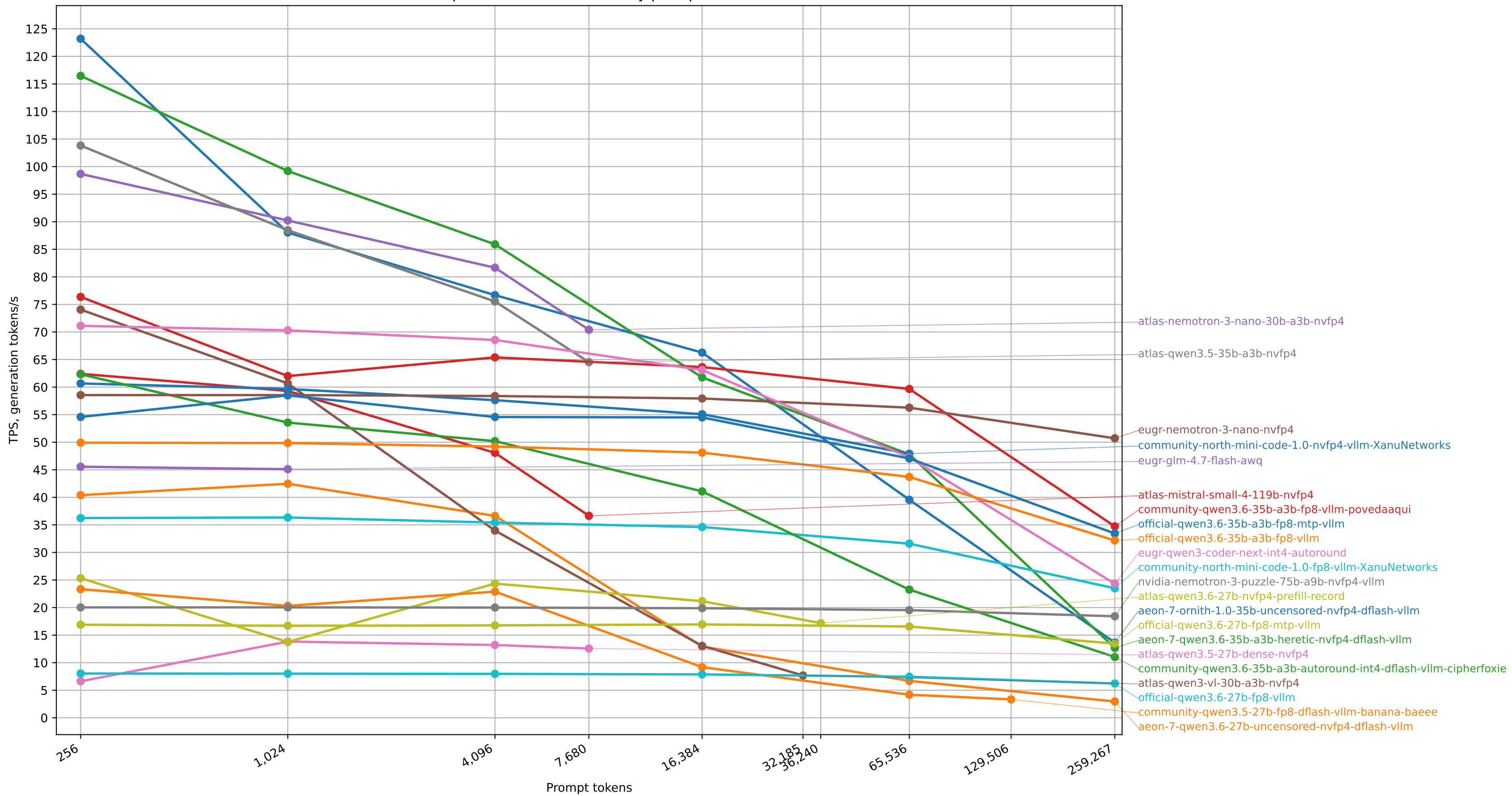
Sparkrun benchmark TPS by prompt size
