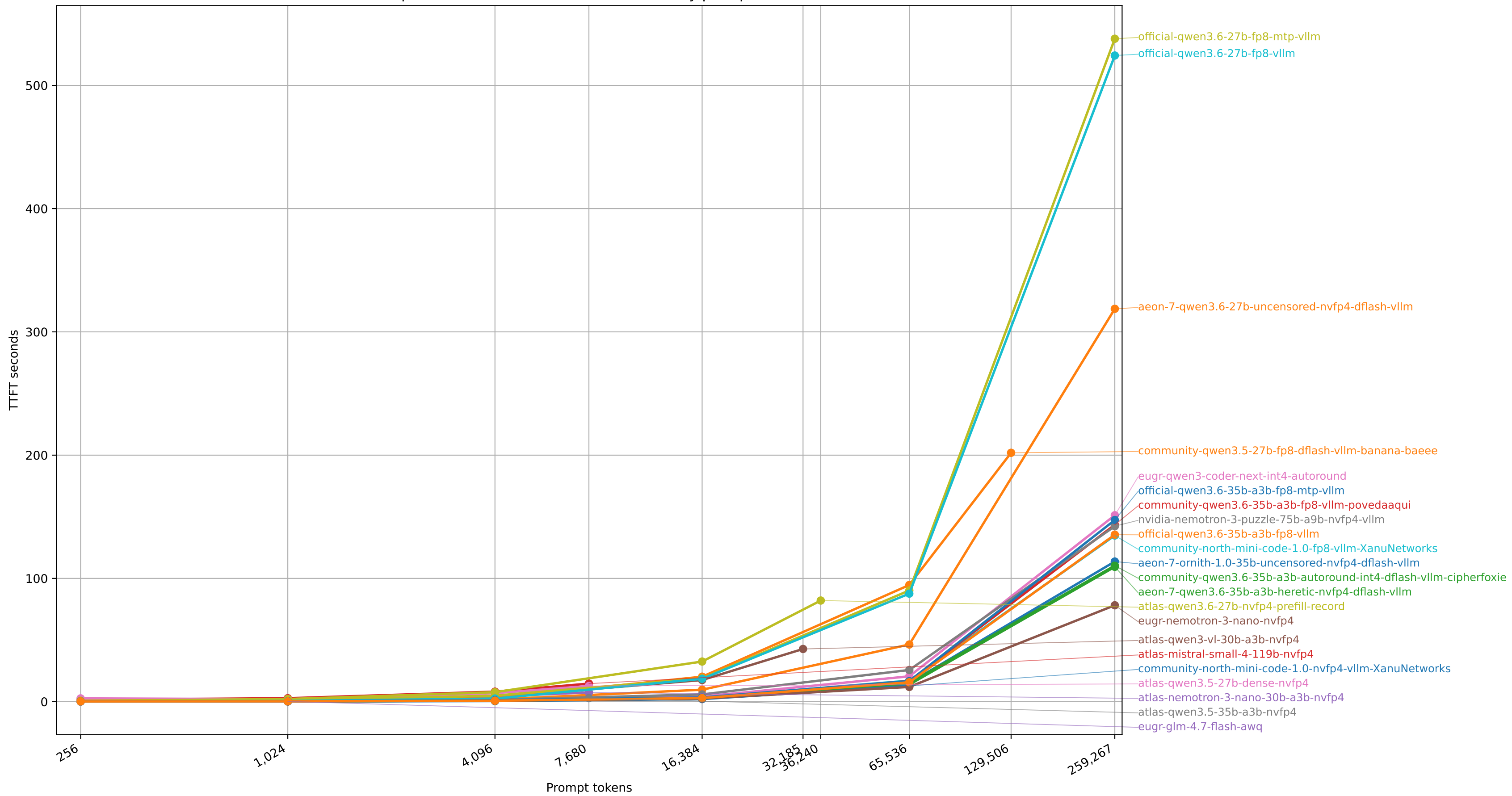
Sparkrun benchmark time to first token by prompt size
